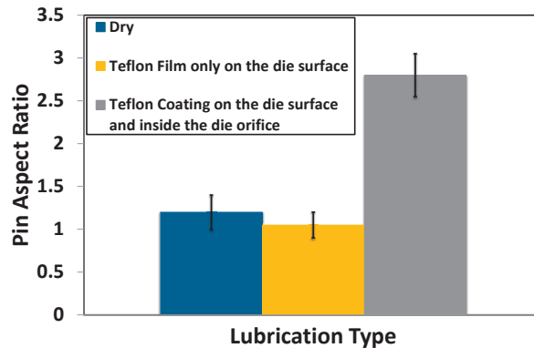
Fig. 2. Effect of solid lubricant (Teflon), coated on different part of the forming tool, on the final pin aspect ratio for the 1.2 mm pin manufacture by the 2.0 mm punch.
