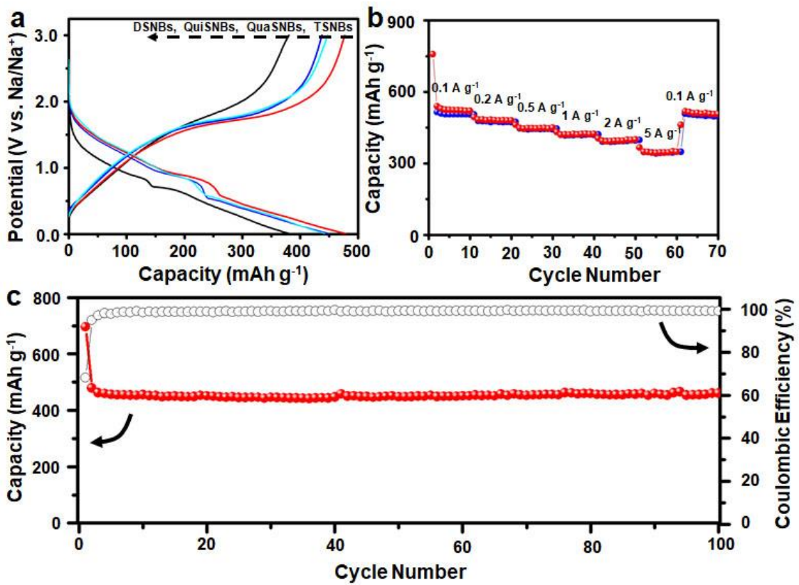
Figure 5. (a) The discharge-charge voltage profiles of cobalt sulfide MSNBs with different shell numbers for the second cycle at the current density of 500 mA g -1 . (b) The rate performance of cobalt sulfide TSNBs at various current densities and (c) cycling performance for 100 cycles at the current density of 200 mA g -1 .
