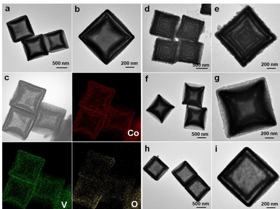
Figure 3. TEM (a, b, d-i) and element mapping (c) images of cobalt divanadate TSNBs (a-c), QuiSNBs (d, e), QuaSNBs (f, g), and DSNBs (h, i).
