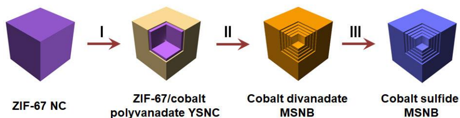
Figure 1. Schematic illustration of the formation process of cobalt sulfide MSNB: I) transformation of ZIF-67 NC to ZIF-67/cobalt polyvanadate YSNC through polyvanadate involved ion-exchange reaction in alkaline media; II) formation of cobalt divanadate MSNB via polyvanadate decomposition and in situ ion-exchange reaction between the released divanadate ions and ZIF-67 core; and III) formation of cobalt sulfide MSNB through a sulfidation reaction.
