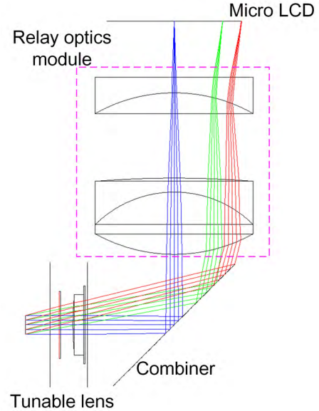
Fig. 5. Optics layout of our near-eye display system.
