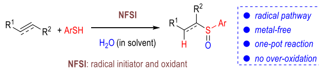
Figure 1 Our strategy of NFSI-enabled selective one-pot access to sulfoxides from alkenes/alkynes and thiols
