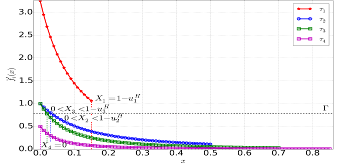
Fig. 2. The plot of \bar{f}'_i(X_i = x) varying x \in \mathbb{R}^+ for the task set in Table II
