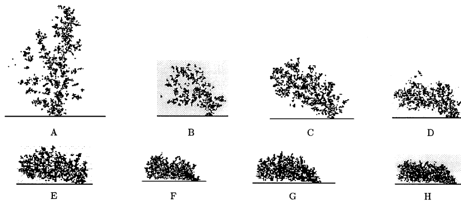
FIG. 3. Slices through the middle (in the x - y plane) of the lattices with the aggregates, the flow is directed from the left to the right. The Péclet numbers for (a)–(h) are given in columns 1–8 of Table I, respectively.
