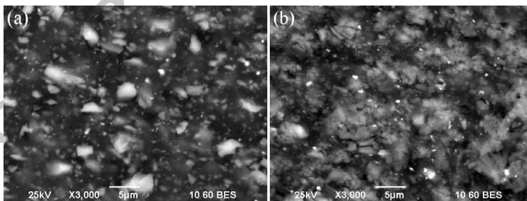
Fig. 5. Typical backscattered electron micrographs of (a) unhydrated and (b) hydrated HNBR-MgO compounds filled with 14% by volume of MgO. The whitish-gray areas
