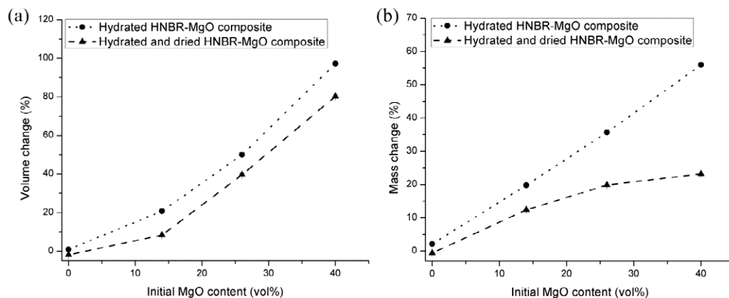
Fig. 2. Plot of change in extent of (a) composite swelling and (b) composite mass change, with MgO filler content of composites
