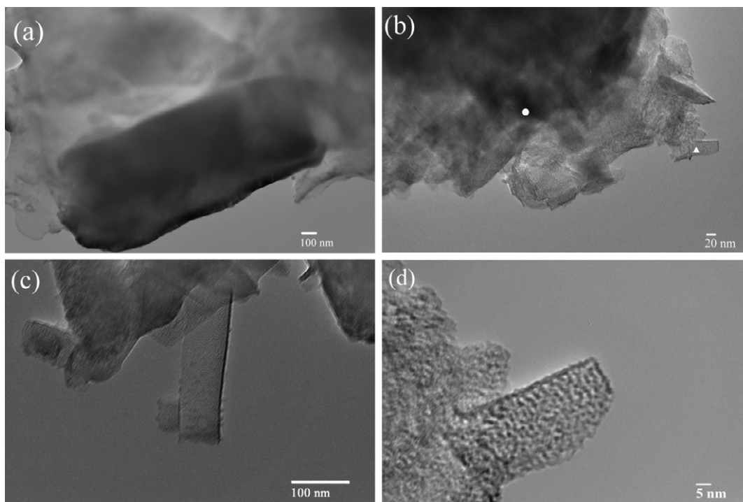
Fig. 6. Typical TEM images of (a) unhydrated composite at 12 000x magnification, (b) hydrated composite at 40 000x magnification, (c) hydrated composite at 30 000x magnification and (d) hydrated composite at 250 000x magnification. These images were obtained using HNBR-MgO composite filled with 40% by volume MgO
