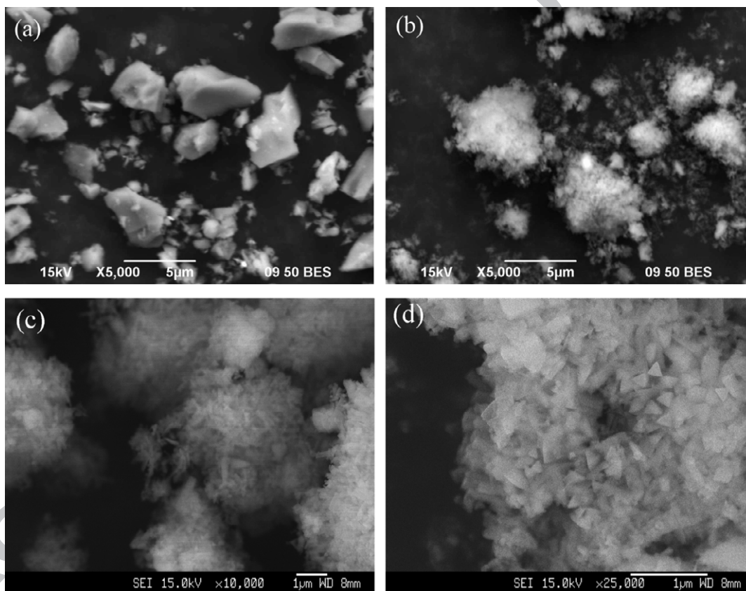
Fig. 3. Typical backscattered micrographs of (a) MgO and (b) Mg(OH) 2 . Secondary electron imaging of Mg(OH) 2 at (c) 10 000 magnification and (d) 25 000 magnification. The white particles are the MgO and Mg(OH) 2 powder while the black areas are the background
