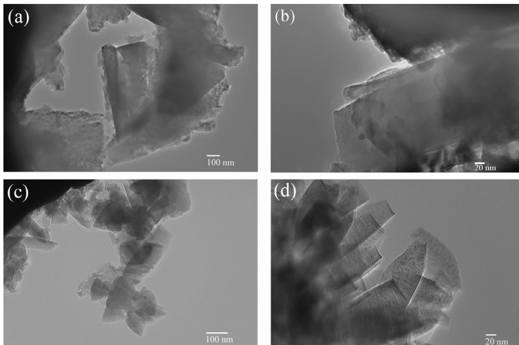
Fig. 4. Typical TEM images of (a) MgO at 15 000x magnification, (b) MgO at 60 000 magnification, (c) Mg(OH) 2 at 25 000x magnification and (d) Mg(OH) 2 at 50 000x magnification
