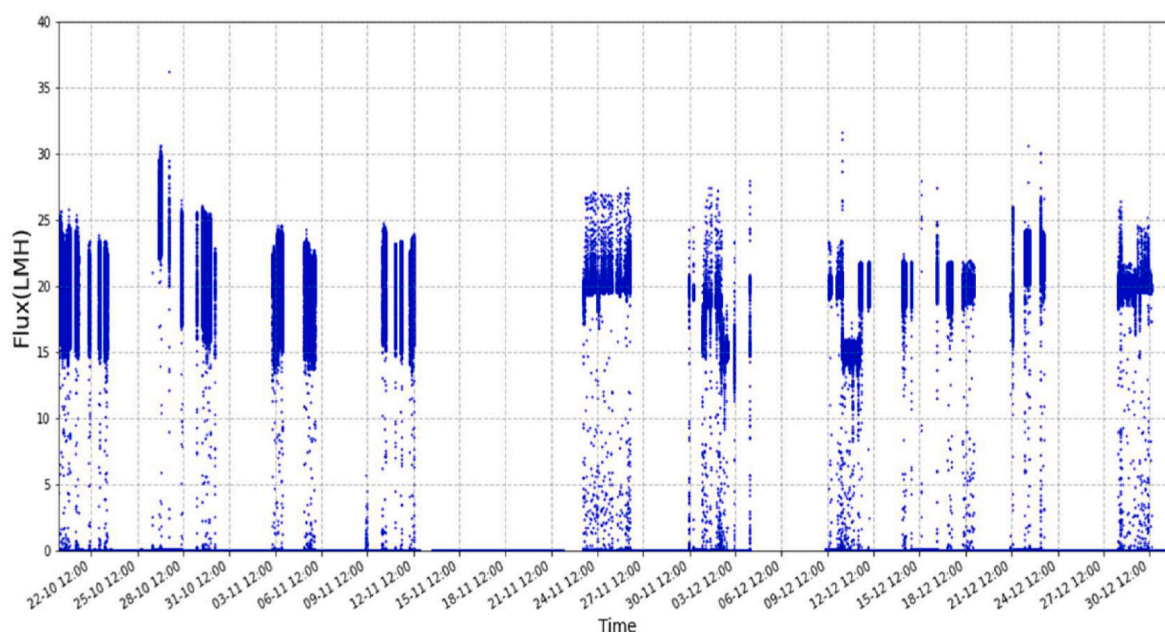
Fig. 5. Flux of dNF40 membranes (in L m^{-2} h^{-1} ) at a pilot at La Zaragozana beer brewery in Spain over a 2-month period. Production stops during the COVID-19 pandemic are the cause of the discontinuous data. Reproduced from [184].
