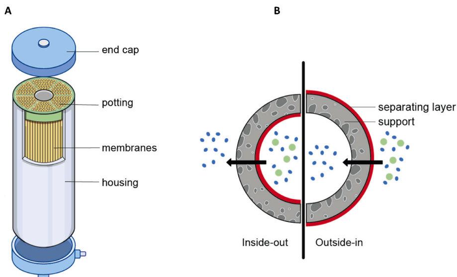
Fig. 2. A) Schematic representation of a hollow fiber module B) Inside-out vs outside-in filtration.
