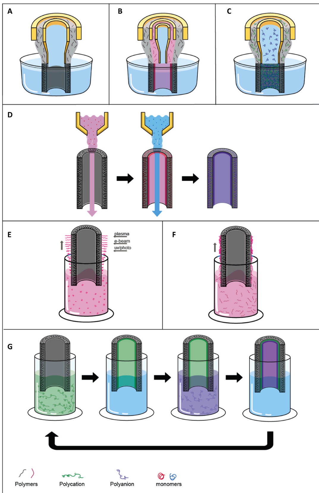
Fig. 1. Methods to fabricate hollow fiber nanofiltration membranes. It should be stressed that most of these methods, save grafting, can be performed on either the inside or the outside of the hollow fiber. For simplicity, only one of these options is displayed per method. A) Single layer phase inversion B) Dual layer phase inversion C) Chemistry in a spinneret D) Interfacial polymerization E) Grafting F) Dip-coating G) Polyelectrolyte multilayers.
