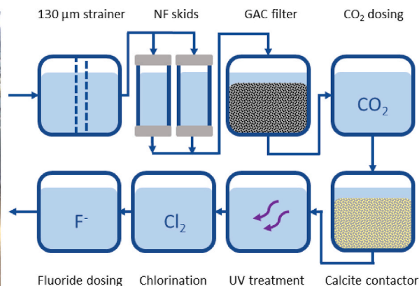
Fig. 7. Full-scale hollow fiber nanofiltration at Ringarooma Valley, Australia. A) Picture of the hollow fiber nanofiltration skids, reproduced from [144] B) Schematic overview of the treatment scheme, image based on information in [144].
