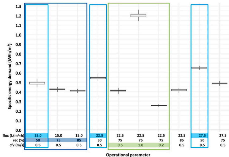
Fig. 4. Impact of operating conditions on the specific energy demand of drinking water filtration. Light blue: increase of flux, dark blue: increase of recovery and green: increase of crossflow velocity. Reprinted with permission from [114]. (For interpretation of the references to colour in this figure legend, the reader is referred to the Web version of this article.)
