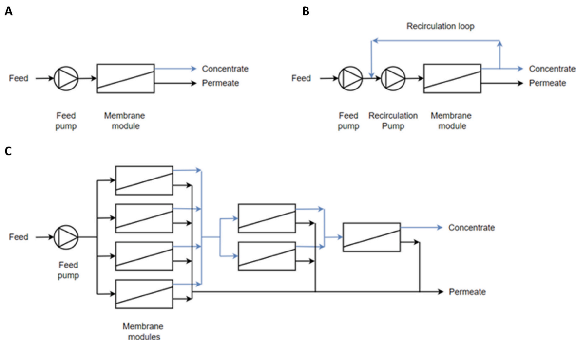
Fig. 3. Several process designs for a plant with hollow fiber nanofiltration modules A) Single-stage, single-pass design B) Single stage feed-and-bleed design C) Christmas-tree staging with seven modules, single-pass design.
