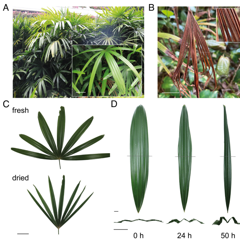
Fig. 1. Corrugated leaf folding in R. excelsa . (A) R. excelsa . Inset : A healthy frond of the plant. (B) A completely dried frond found in nature shows the folded morphology. The Inset shows the zoomed-in image of the folded leaves. (C) A frond of R. excelsa before and after air drying in the lab for 72 h. (D) A leaf after different periods of air drying. The Bottom panel shows the corresponding transverse section of the leaf. [Scale bars, 5 cm in (A–C) and 1 cm in (D).]
