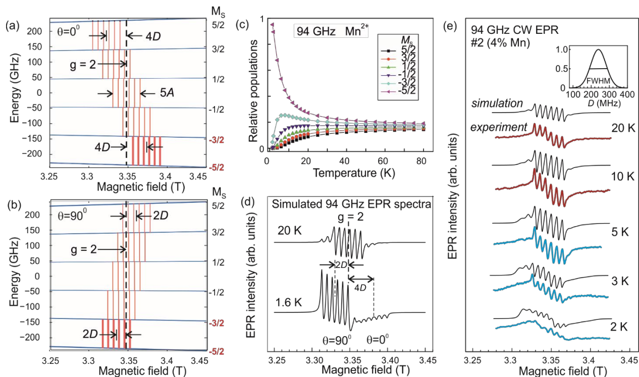
Figure 4. Energy levels of the \text{Mn}^{2+} ion ( S = 5/2 , I = 5/2 ) for a magnetic field oriented parallel (panel a) and perpendicular (panel b) to the NPL [001] axis. (c) Calculated relative populations of the six fine-structure levels of \text{Mn}^{2+} ions at the magnetic field corresponding to EPR at 94 GHz. The sum of the relative populations is 1 for any temperature. (d) Simulated EPR spectra at 94 GHz for a powder sample containing axial \text{Mn}^{2+} ions, A = 7 mT, D = 9 mT. (e) Comparison of the experimental CW EPR spectra measured in sample #2 at 94 GHz for different temperatures, and simulated EPR spectra of axial \text{Mn}^{2+} centers with the parameters given in the text. When recording these spectra, the phase of the IQ detector was adjusted to obtain EPR signals in the form of a derivative of the absorption line. The inset shows the Gaussian distribution of the D value used to simulate the spectra.
