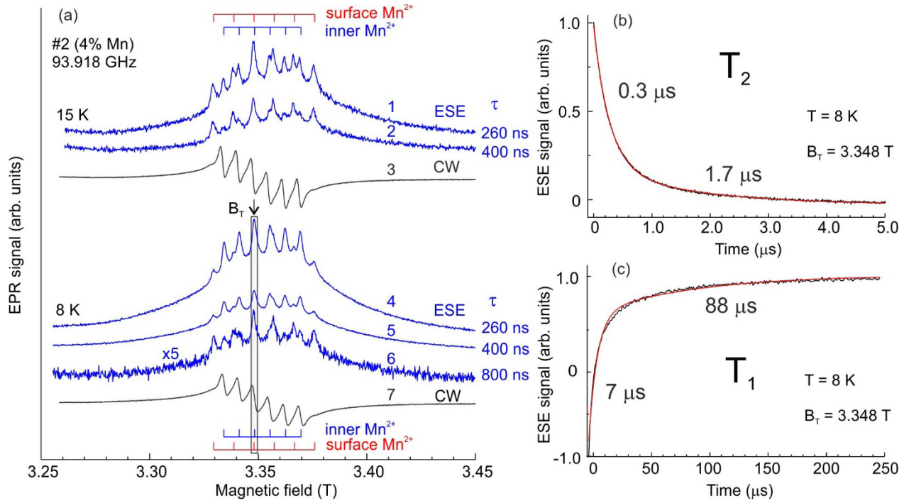
Figure 3. (a) EPR spectra of sample #2 measured at 8 K and 15 K on a Bruker spectrometer in CW (spectra 3 and 7) and pulsed mode. The ESE-detected EPR (spectra 1, 2, 4–6) were measured using \pi/2 - \tau - \pi pulse sequences with the \pi/2 pulse duration of 16 ns and \tau = 260 ns (1 and 4), 400 ns (2 and 5) and 800 ns (6). Experimental ESE decay (or recovery) curves to measure the spin-spin relaxation time T_2 (b) and spin-lattice relaxation time T_1 (c) at T = 8 K. Bi-exponential fits are shown by the red lines, the measurements are taken in a magnetic field B_T = 3.348 T as marked in Figure 3a by the arrow.
