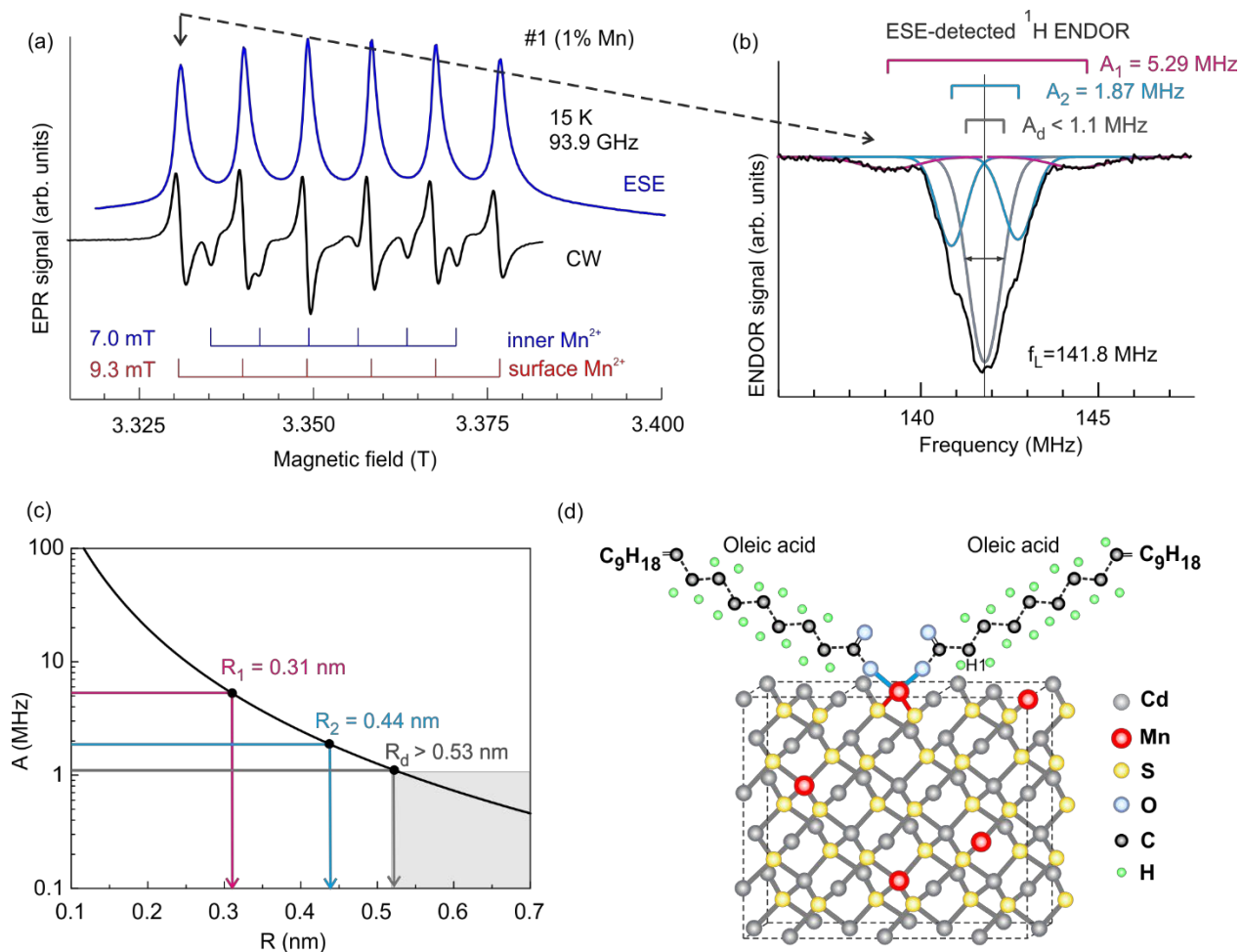
Figure 5. (a) EPR spectra recorded at 93.9 GHz and T = 15 K on sample #1: (top) ESE-detected EPR and (bottom) CW EPR. (b) ESE-detected ENDOR spectrum measured in a magnetic field corresponding to the EPR of the surface \text{Mn}^{2+} ions, f_L is the Larmor frequency of the ^1\text{H} nucleus in a magnetic field marked with the arrow in panel (a). (c) Dependence of the hydrogen hyperfine interaction constant A_i on the distance R between the \text{Mn}^{2+} electron spin and the i -th ^1\text{H} nucleus. Circles mark the A_i values determined from the ENDOR spectrum. (d) \text{Mn}^{2+} -doped CdS shell of the NPL and oleic acid ligands, which passivate the surface \text{Mn}^{2+} ion. a = 0.5832 nm is the lattice constant. The hydrogen atoms marked as H1, H2, and H3, are located at the distances from a \text{Mn}^{2+} ion that correspond approximately to the distances obtained from the ENDOR spectrum.
