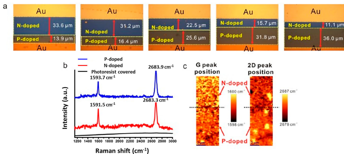
Figure 4. (a) Optical images of the graphene p-n junctions, highlighting both the p- and n- regions. (b) Raman spectra of undoped (P-type, blue) and o -MeO-DMBI- (6 nm)-doped (red) and photoresist-covered (black) CVD-graphene. (c) Maps of G and 2D peak position in the junction region. [49].
