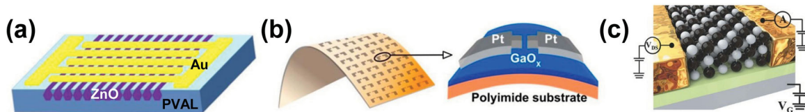
Figure 18. (a) Device structure of ZnO photodetector [110]. (b) Device structure of amorphous GaO x thin-film photodetector [112]. (c) Illustration of SnTe NM photodetector [113].
