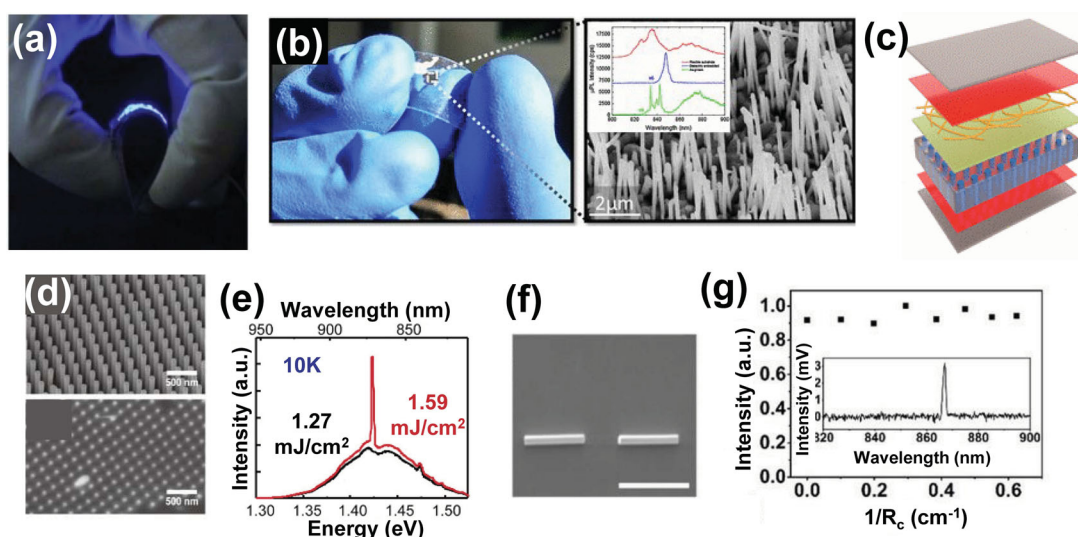
Figure 10. (a) Photographs of InGaN/GaN MQW LED in operation under bending [81]. (b) Image of flexible GaAs NW LED along with SEM image of NWs and emission spectrum of the device [85]. (c) Structure of ZnO/Si NW LED [86]. (d) SEM image of GaAs NWs with InGaAs/GaAs QDs and (e) the output spectrum of the device [87]. (f) SEM image of InP NWs and (g) output spectrum along with the output light intensity vs. the bending radius [88].
