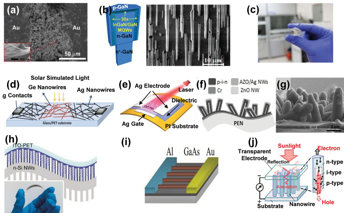
Figure 9. (a) SEM image of ZnO NWs (center) with Au contacts [73]. (b) Illustration of core-shell InGaN/GaN NW structure and SEM image of InGaN/GaN NWs [74]. (c) Image of flexible Si NW on PET [75]. (d) Illustration of flexible photodetector with Ge NWs as the active material along with Ag NWs and SWNTs as charge transport layers [76]. (e) Illustration of CNT photodetector on flexible PI substrate [77]. (f) Device structure of hybrid ZnO/a-Si NW flexible photodetector on PEN substrate and (g) SEM image of the structure [78]. (h) Si NW device structure on flexible ITO-PET substrate along with image of the device under bending [79]. (i) Device structure of GaAs NW photodetector. (j) Schematic of InP NW photodetector [80].
