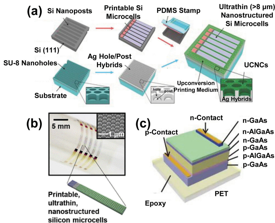
Figure 19. (a) Fabrication procedure for patterned Si nanostructure solar cells. (b) Image of printable nanostructured Si wrapped on glass rod [114]. (c) Device structure of flexible GaAs NM solar cell [115].
