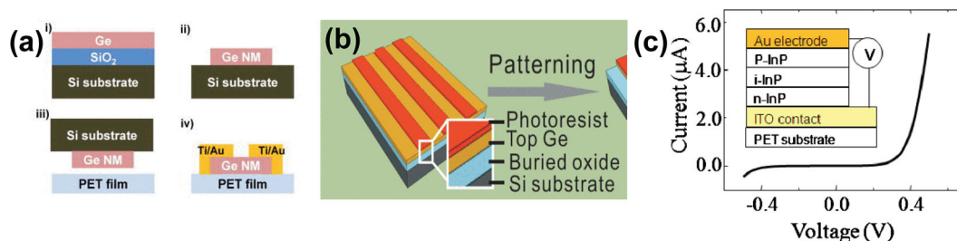
Figure 16. (a) Device structure of Ge NM photodetector on PET [64]. (b) Device structure of Ge photodetector [107]. (c) Device structure and current-voltage characteristics of InP NM photodetector [108].
