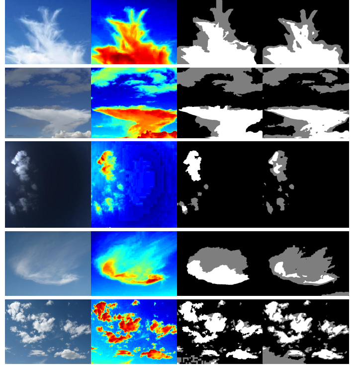
Fig. 1: Five image samples, from left to right: Original image from HYTA database; probabilistic cloud detection using [14]; 3-level ground-truth; 3-level labels generated using our proposed approach.
