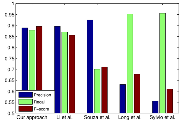
Fig. 3: Evaluation results for binary semantic labeling of the images in the HYTA database.
