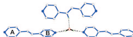
Figure 5. The crystal superstructure of 4,4'-vinylenedipyridine.
