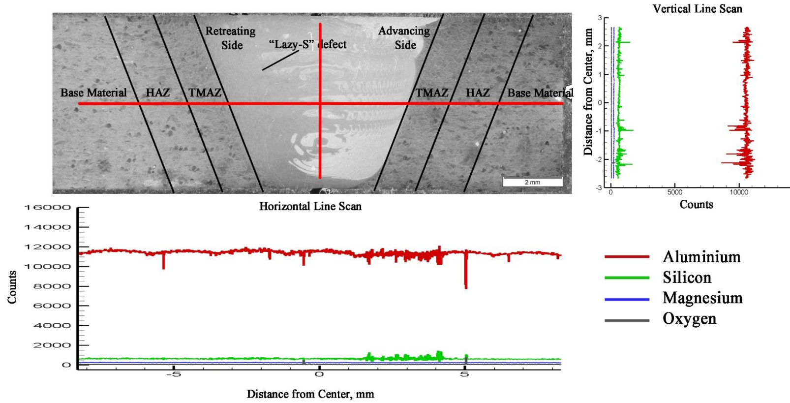
FSW with low heat input with low tilt angle of SLM of AlSi 10 Mg with high VED.
