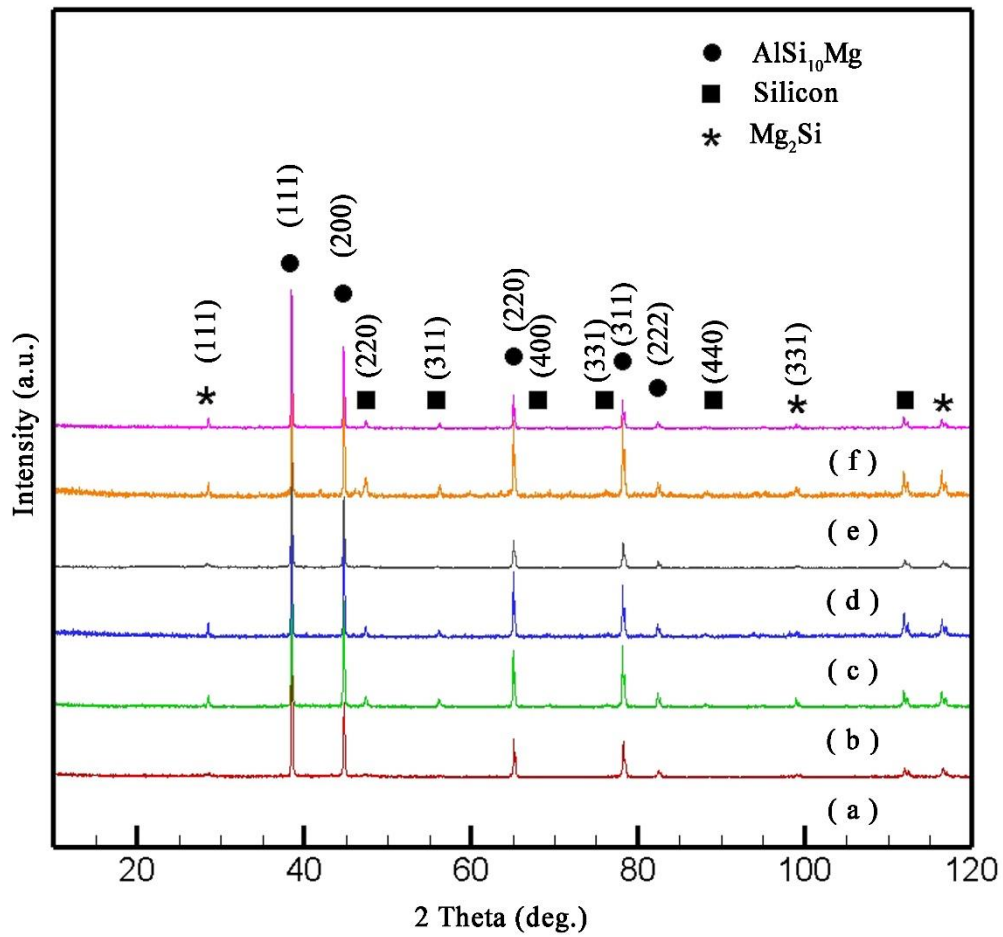
Figure 7-4 X-Ray diffraction pattern of the SLM of \text{AlSi}_{10}\text{Mg} with high VED (a) as-received, (b) FSW with low heat input, (c) FSW with high heat; SLM of \text{AlSi}_{10}\text{Mg} with low VED (d) as-received, (e) FSW with low heat input, (f) FSW with high heat input.
