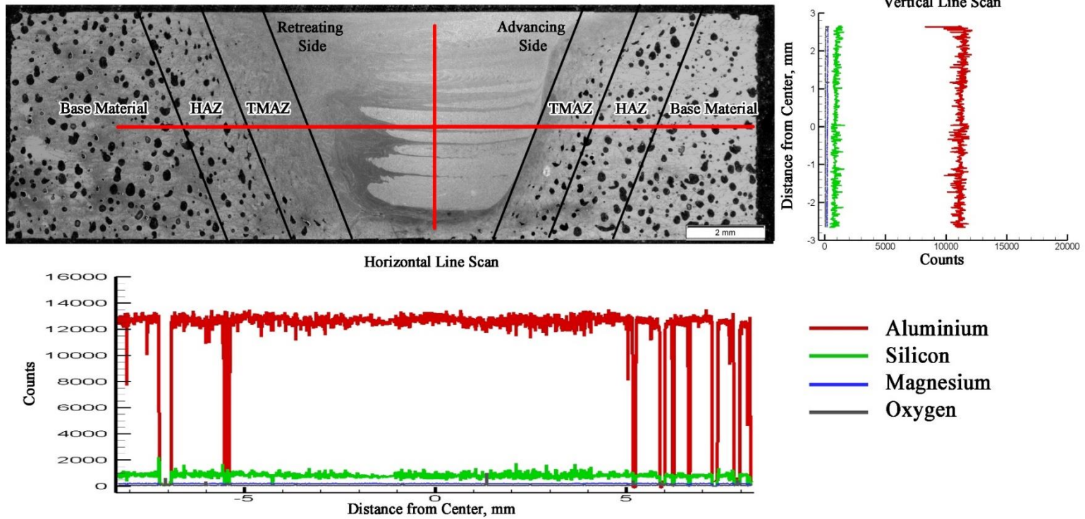
FSW with low heat input of SLM of AlSi 10 Mg - 5% wt. nAl 2 O 3 with high VED.
