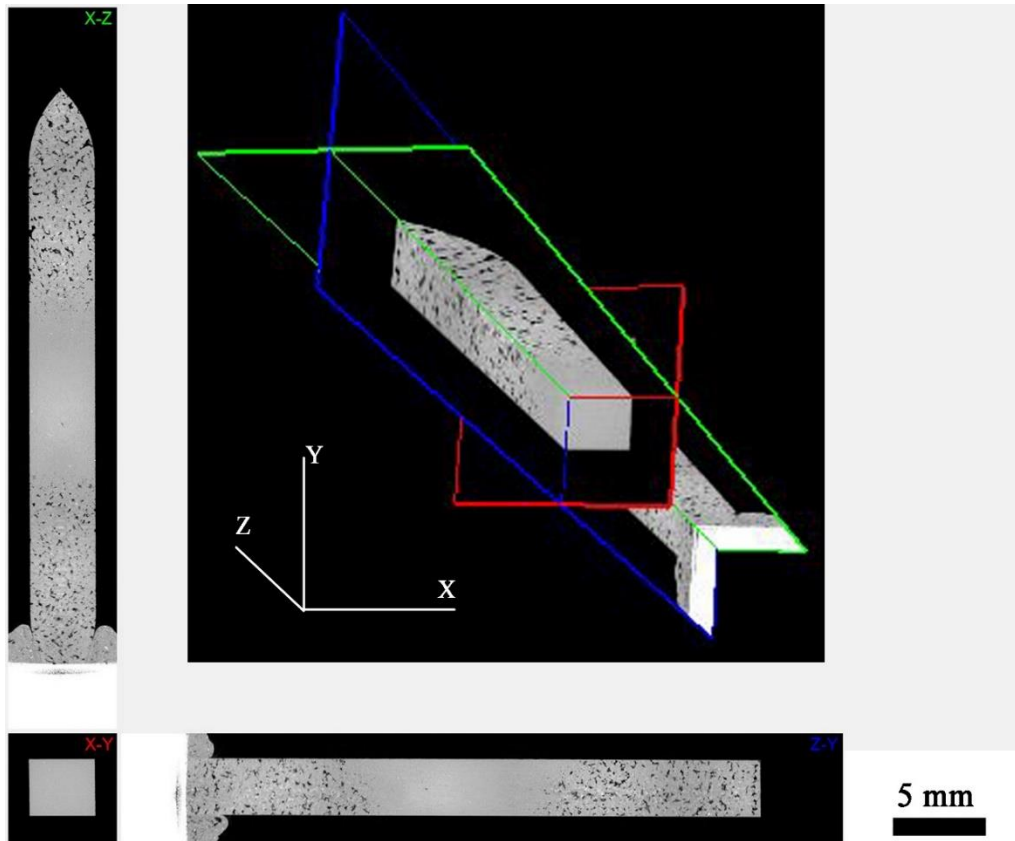
FSW with high heat input of SLM of AlSi 10 Mg - 5% wt. nAl 2 O 3 with high VED.
