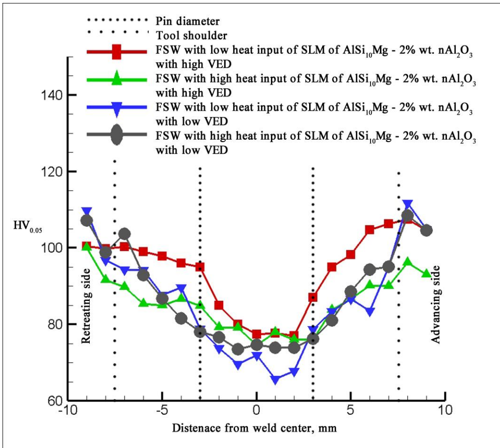
Figure 7-23 Hardness profile of FSWed samples of SLM fabricated \text{AlSi}_{10}\text{Mg} - 2% wt. \text{nAl}_2\text{O}_3 composites.
