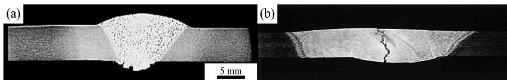
Figure 2-11 Tungsten inert gas (TIG) butt welding of 6mm plate showing trapped porosity in the weld region, and hot cracking in AA6082 with 4043 filler metal [16].
