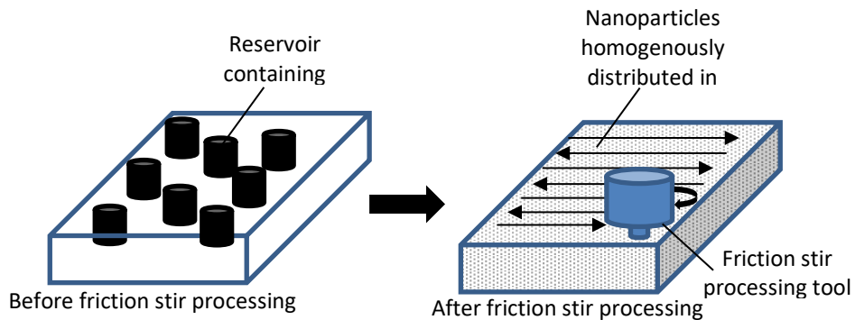
Figure 4-1 Schematic diagram showing how the FSP of the nanocomposites.
