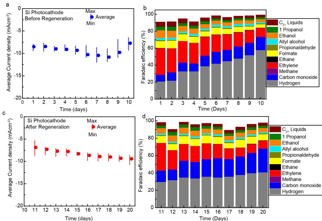
Fig. 4. Stability measurement of a textured silicon photocathode with an integrated Ag-supported dendritic Ag catalyst at -0.4 V vs RHE in 0.1 M \text{CsHCO}_3 electrolyte solution under simulated 1-sun illumination. Simulated diurnal cycling was performed with 10 hrs light on and 14 hrs light off. The electrolyte was changed after each daily measurement of the liquid products. a. Daily average photocurrent over 10 days of the Si photocathode before regeneration of the catalyst. Current density data points were averaged over a day; the vertical line indicates the maximum and minimum current density on that day. b. \text{CO}_2\text{R} product distribution with time. c. Daily average/high/low photocurrent of the Si photocathode after Cu catalyst regeneration. d. \text{CO}_2\text{R} product distribution with time of the regenerated photocathode.
