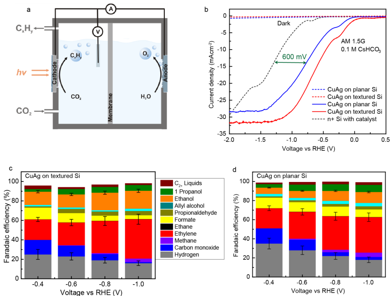
Fig. 3. a. Schematic of the membrane-separated PEC cell. b. Photocurrent-potential curve of Si photocathodes in three electrode configuration and under dark and simulated 1 Sun (AM 1.5G, 100 mW cm -2 ) illumination. The grey dotted line shows data from the dark cathode (Ag-supported dendritic Cu on n + /n-Si), while the solid grey double sided arrow shows the generated photovoltage (~600 mV) for the planar photocathode. c. Faradaic efficiency of textured Si photocathode with Ag-supported dendritic Cu. d. Faradaic efficiency of CuAg deposited planar Si photocathode with Ag-supported dendritic Cu. C 2 + liquids in Fig. 3c and Fig. 3d refer to acetate, acetaldehyde, glyoxal, glycolaldehyde, ethylene glycol and hydroxyacetone. The electrolyte in all cases was in 0.1 M CsHCO 3 , pH 6.8. Error bars show the standard deviation from repeated experiments. See ESI Figs. S5 and S6 for examples of raw data used to generate the FE plots.
