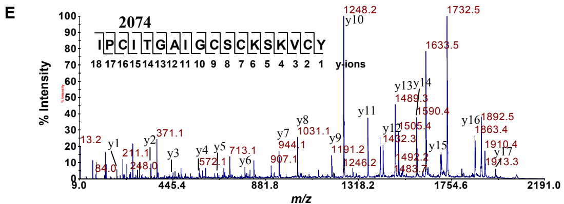
Figure 57. MS/MS sequencing of clotide T1. (A) Trypsin digestion of S-alkylated clotide T1 yielded 812- and 2657-Da fragments; and chymotryptic digestion yielded 1395- and 2074-Da fragments. (B-E) MS/MS spectra of digested fragments. Analysis of these spectra gave overlapping sequences indicative of a cyclic backbone of clotide T1.
