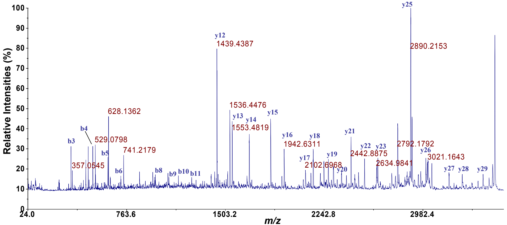
Figure 11. MS/MS spectrum of linearized S-alkylated hedyotide B7 upon digestion with (A) trypsin and (B) endoproteinase Glu-C. Complete sequence coverage of 30 residue cyclotides was obtained in single spectrum.
