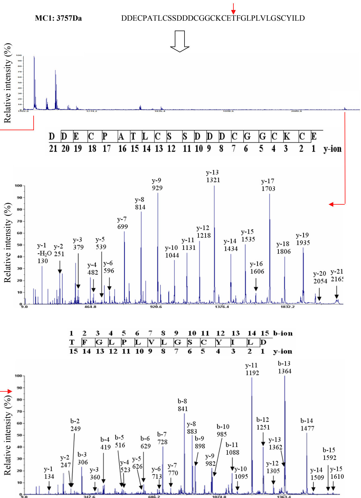
Figure 37. MS/MS sequencing of morintide C1. A. Enzymatic cleavage of morintide C1 by EndoGlu-C. The resultant ions were fragmented by MS/MS. B. MS/MS spectra of the 2165-Da-fragment. The y-ion sequence is shown. C. MS/MS spectra of the 1610-Da-fragment. Both b- and y-ion series are shown. Combining both sets of sequences gave the overall sequence of MC1 as DDECPATLCSSDDDCGGCKCETFGLPLVLGSCYILD.
