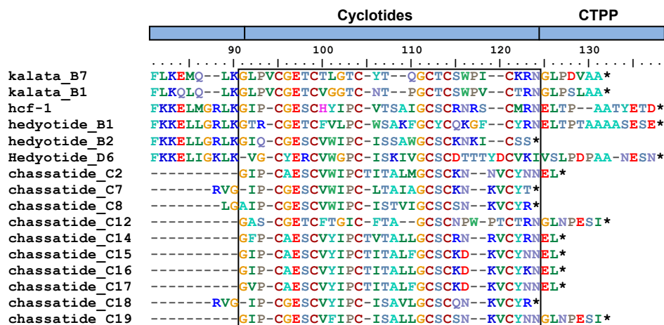
Figure 29. Multiple sequence alignment of chassatide precursors with kalata B1, kalata B7, hcf-1, hedyotide B1, B2 and D6 precursors. The mature cyclotide domains are boxed. Asterisk indicates stop codon.
