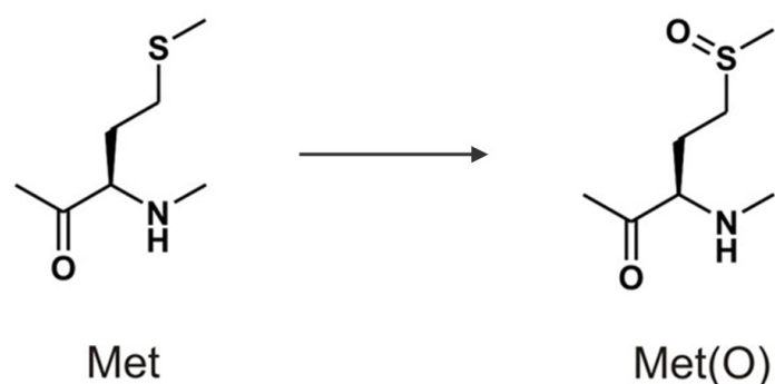
Figure 31. Oxidation of methionine to methionine sulfoxide.
