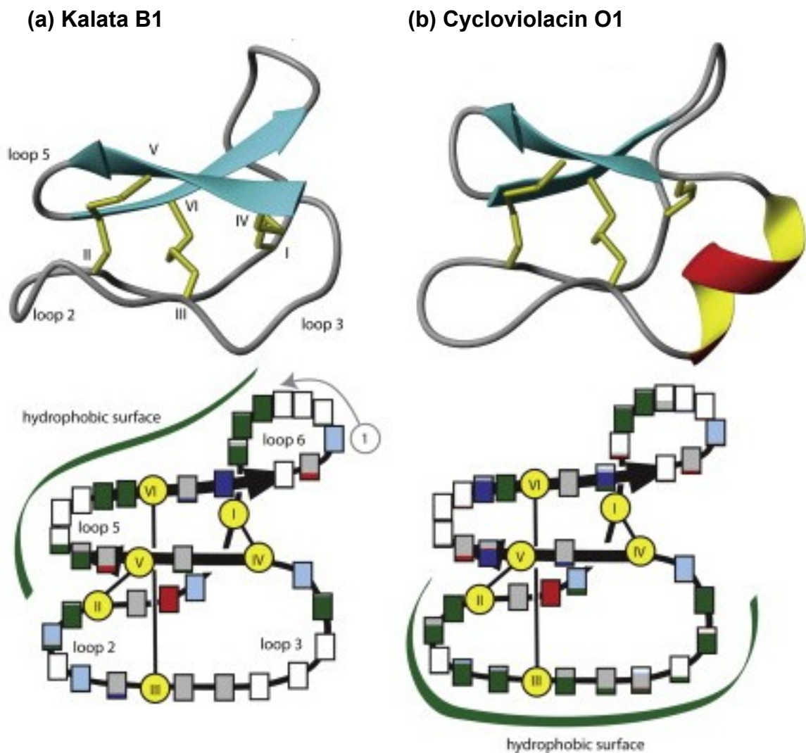
Figure 3. Representative structures of Möbius and bracelet cyclotides. (a) Kalata B1 has a Möbius structure characterized by a cis-Pro residue in loop 5 that leads to a conceptual twist. (b) Cycloviolacin O1 of the bracelet family. About two-third of cyclotides belong to this family. Figure taken from Wang et al. [29].
