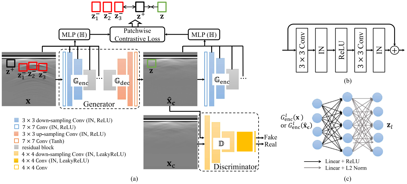
Fig. 3. (a) Architecture of the contrastive learning-based GAN for estimating the clutter-only B-scan \hat{\mathbf{x}}_c from the input noisy B-scan \mathbf{x} . (b) Structure of the residual block. (c) Structure of the multilayer perceptron (MLP) network to obtain the projected features via \mathbf{z}_l = \mathbb{H}_l(\mathbb{G}_{\text{enc}}^l(\mathbf{x} \text{ or } \hat{\mathbf{x}}_c)) . Note that “Conv,” “IN,” “ReLU,” “Tanh,” “LeakyReLU,” “Linear,” and “L2 Norm” represent the convolution, instance normalization, ReLU activation, Tanh activation, Leaky ReLU activation, fully connected layer, and L2 normalization, respectively.
