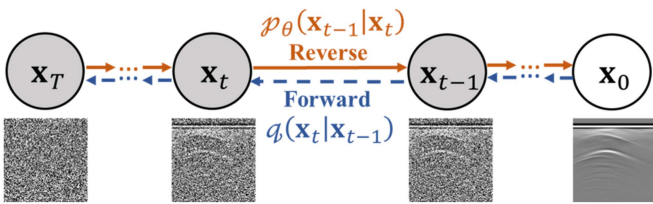
Fig. 2. Chain transitions of the forward and reverse diffusion process for generating the GPR B-scan.
