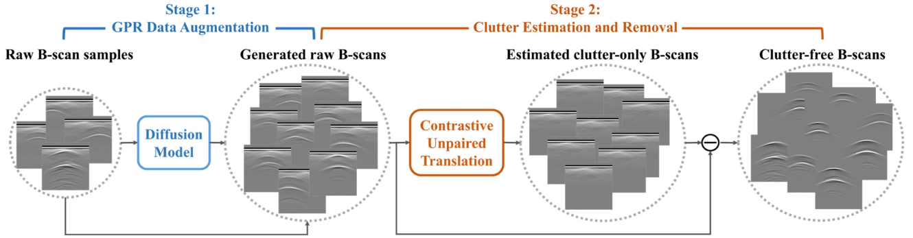
Fig. 1. Overview of the proposed two-stage framework ULCR-Net for removing clutter in GPR images based on unsupervised learning.
