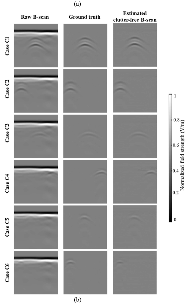
Fig. 9. (a) Schematic of the simulation scenario of the complicated surface with rough ground, water puddles, and grass blades. (b) Imaging results of the clutter removal for complex scenarios. Cases C1–C3 represent three testing scenarios in which the depth range of the object center is randomly selected from [0.10, 0.25] m. Cases C4–C6 represent three new scenarios in which the depths of the object's upper surface are 4, 2, and 1 cm, respectively.
