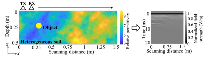
Fig. 4. Typical simulation scenario for generating the training dataset and regular testing dataset with one cylindrical object and the obtained B-scan via the GPR scanning.
