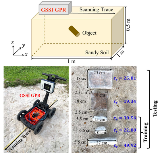
Fig. 11. Experiment setup for collecting real measurement data. Only single-cylinder-object scenarios are used for training. New scenarios with box-shaped objects and multiple objects are used to test network generalizability.
