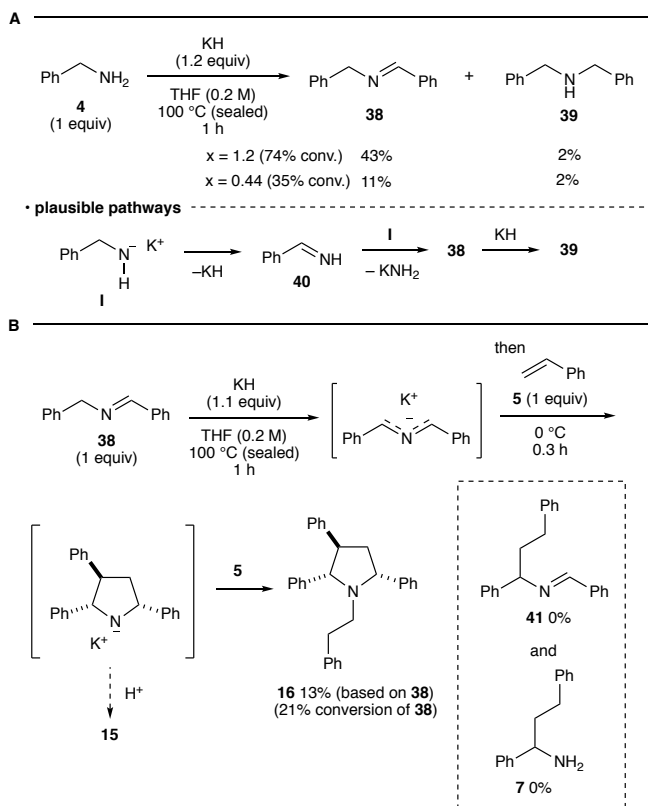
Scheme 8. Reactivity of benzylamine ( 4 ) and N -benzylimine 36 in the presence of KH.
