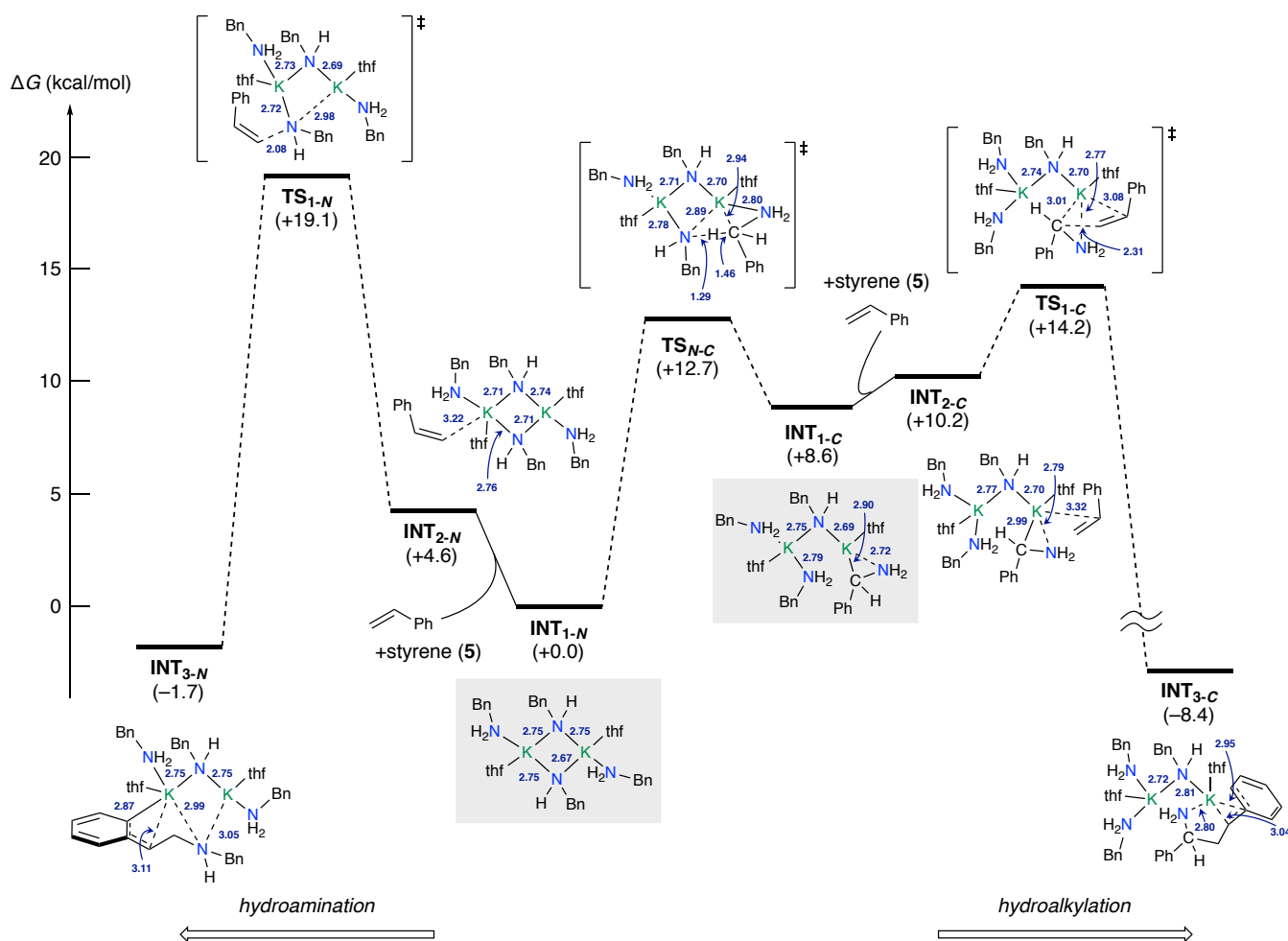
Scheme 11. DFT calculations on the hydroamination and hydroalkylation reactions of modeled dimeric species with styrene ( 5 ). Energy changes and bond lengths at the M06-2X/6-311++G*/SMD(THF)//M06-2X/6-31+G* level of theory are shown in kcal/mol and Å, respectively.
