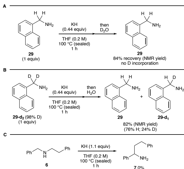
Scheme 9. Deuterium labelling experiments with 27 and reactivity of 6 .
