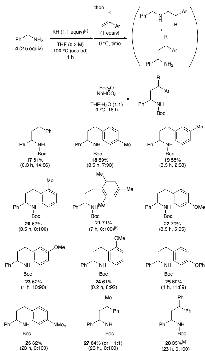
Scheme 7. Scope of benzylamines.
