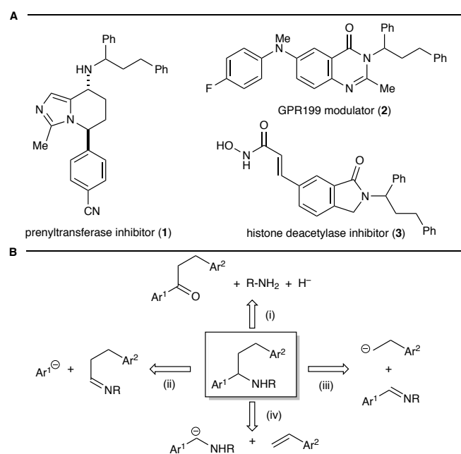
Scheme 1. (A) Bioactive molecules having a 1,3-diarylpropylamine moiety. (B) Retrosynthetic approaches toward 1,3-diarylpropylamines.
