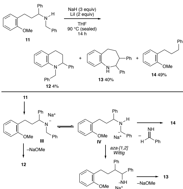
Scheme 5. Observation of equilibrium between sodium amide and benzylic anion species.
