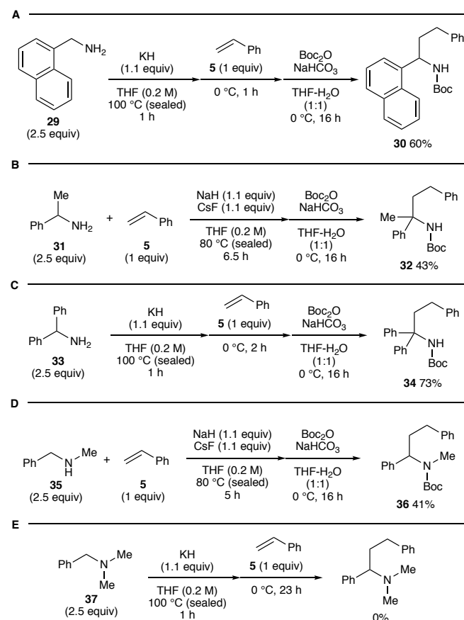
Scheme 7. Scope of benzylamines.
