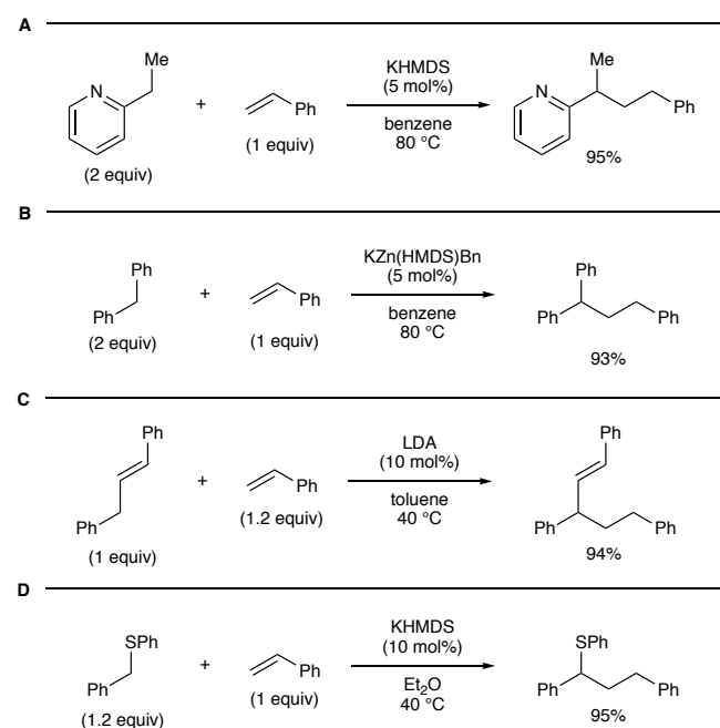
Scheme 2. Addition of benzylic carbanion to styrenes.
