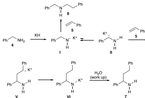
Scheme 10. Proposed mechanisms.
