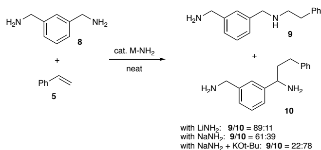
Scheme 4. Counter cation effect in hydroamination/alkylation of styrene ( 5 ) with 1,3-phenylenedimethaneamine ( 8 ).
