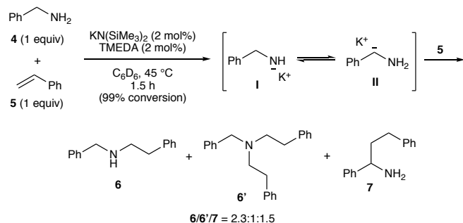
Scheme 3. Observation of hydroalkylation of styrene ( 5 ) with benzylamine ( 4 ).
