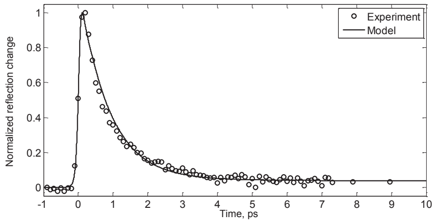
Fig. 4 Decay kinetics of the reflection change at 632 nm from 300 \mu\text{m} gold plated quartz substrate after the excitation with 350 nm 65 fs laser pulse and theoretical curves for penetration depth \kappa=3.0 nm corresponding to electron-phonon relaxation time equals 0.9 ps.
