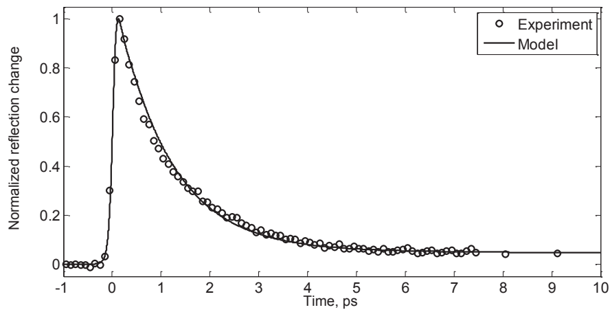
Fig. 3 Decay kinetics of the reflection change at 590 nm from 300 \mu\text{m} gold plated quartz substrate after the excitation with 350 nm 65 fs laser pulse and theoretical curves for penetration depth \kappa=3.8 nm corresponding to electron-phonon relaxation time equals 1.15 ps.
