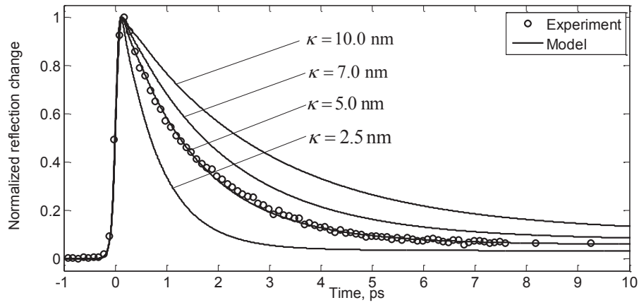
Fig. 2 Decay kinetics of the reflection change at 561 nm from 300 \mu\text{m} gold plated quartz substrate after the excitation with 350 nm 65 fs laser pulse and theoretical curves for different penetration depths \kappa .
