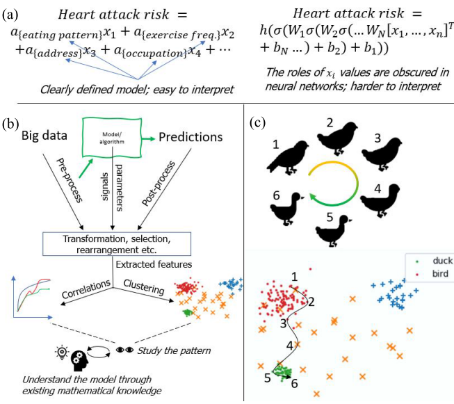
Fig. 5. Overview of methods whose interpretability depend on interpreting underlying mathematical structure. (a) Predefined models. Modeling with clear, easily understandable model, such as linear model can help improve readability, and hence interpretability. On the other hand, using NN could obscure the meaning of input variables. (b) Feature extraction. Data, predicted values, signals, and parameters from a model are processed, transformed, and selectively picked to provide useful information. Mathematical knowledge is usually required to understand the resulting pattern. (c) Sensitivity. Models that rely on sensitivity, gradients, perturbations, and related concepts will try to account for how different data are differently represented. In the figure, the small changes transforming the bird to the duck can be traced along a map obtained using clustering.
