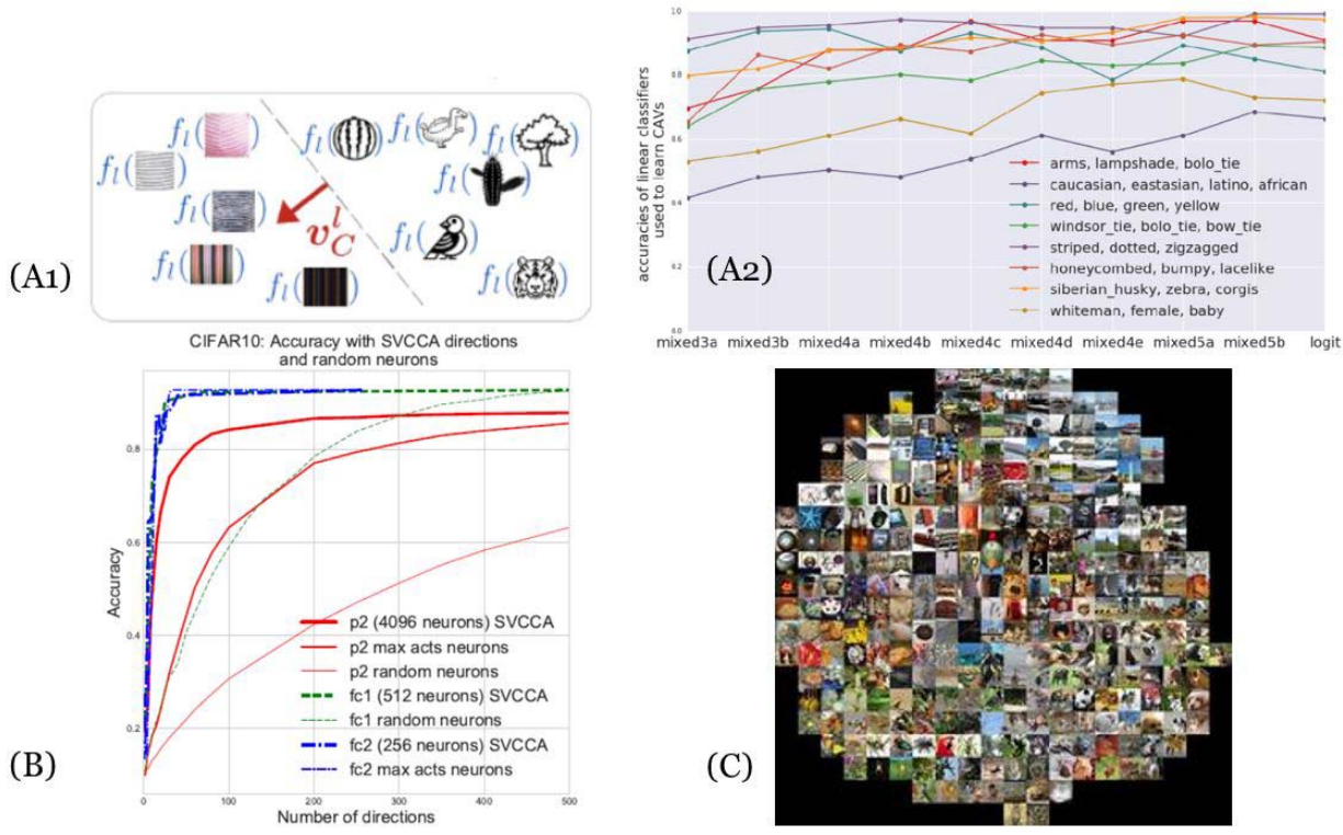
Fig. 4. (a1) TCAV [96] method finds the hyperplane CAV that separates concepts of interest. (a2) Accuracies of CAV applied to different layers supports the idea that deeper NN layers contain more complex concepts, and shallower layers contain simpler concepts. (b) SVCCA [97] finds the most significant subspace (direction) that contains the most information. The graph shows that as few as 25 directions out of 500 are enough to produce the accuracies of the full network. (c) t-SNE clusters images in meaningful arrangement, for example, dog images are close together. Figures (a1) and (a2) are used with permission from the authors Been Kim; figure (b) and (c) from Maithra Raghu and Jascha Sohl-dickstein.
