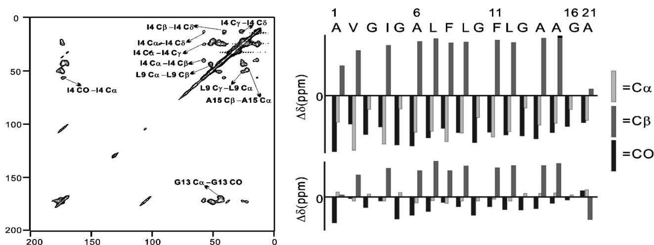
Figure 5: (left panel) 2-D ^{13}\text{C} - ^{13}\text{C} PDSO (Proton-Driven Spin Diffusion) spectrum of membrane associated 23-residue long HIV fusion peptide in solid state. (right panel) Secondary chemical shift of ^{13}\text{C}\alpha , ^{13}\text{C}\beta and ^{13}\text{C}=\text{O} of residues of HIV fusion peptide. The figure was adapted with permission from reference 58. Copyright (2008) American Chemical Society.
