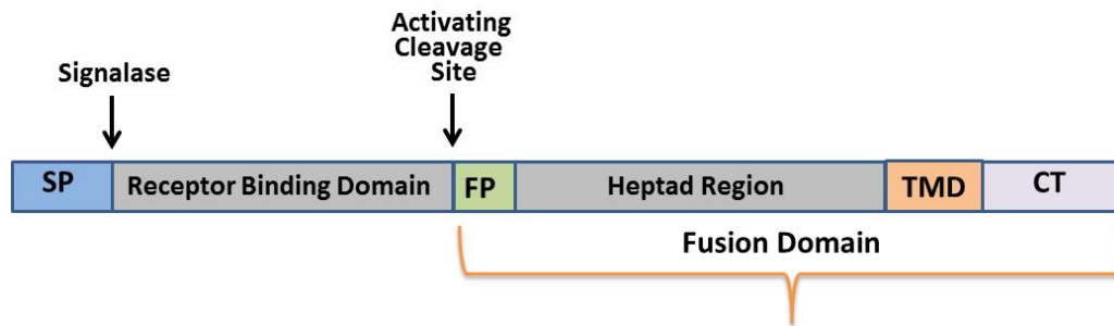
Figure 2. The schematic representation of viral fusion protein.
