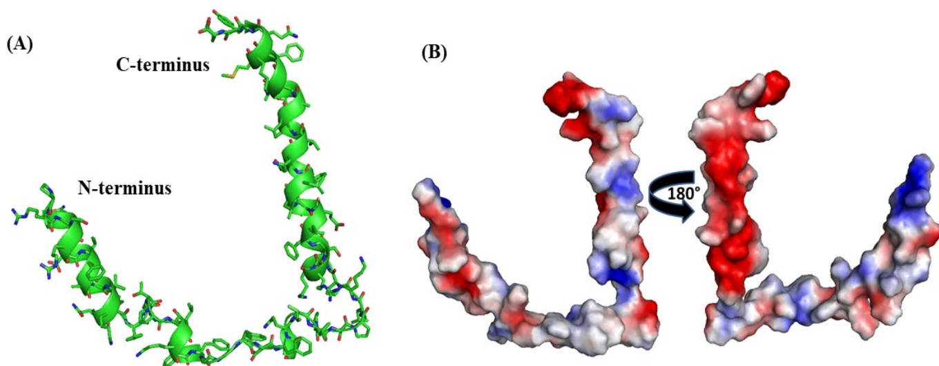
Figure 9. (A) Ribbon representation of 3-D structure of LFP of SARS-CoV-1 showing discretely folded helices. (B) Electrostatic potential surface of LFP, positively charged, negatively charged and uncharged amino acids are marked as blue, red and white color.
