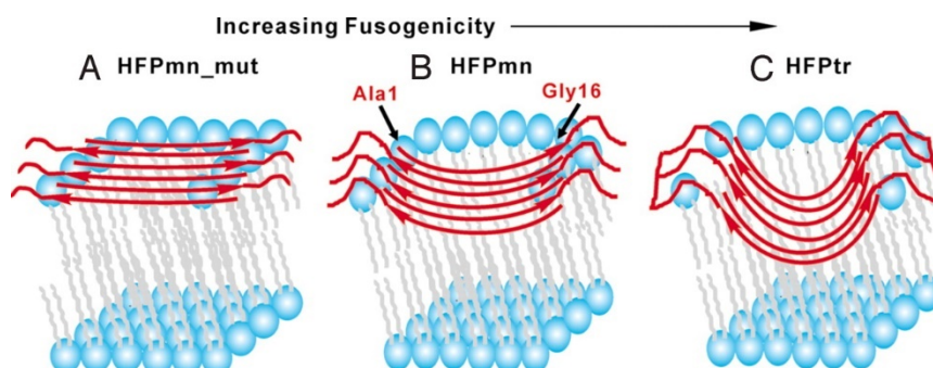
Figure 6: Schematic models of \beta -sheet assembly and localization of HIV-1 gp41 FP in lipid bilayer. HFP mn-mut , HFP mn , HFP tr represent mutated inactive FP, WT FP and cross-linked FP, respectively. The figure has been reproduced from ref 54 with permission.
