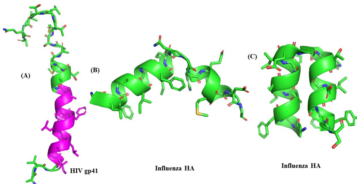
Figure 4: Ribbon representation of micelle bound structures of fusion peptides (A) HIV-1 gp41 (pdb 2ARI), (B) influenza HA (pdb 1IBN) and (C) full length influenza HA (pdb 2KXA). The N-terminal helical segment of HIV-gp41 inserted into micelle has been colored in purple.
