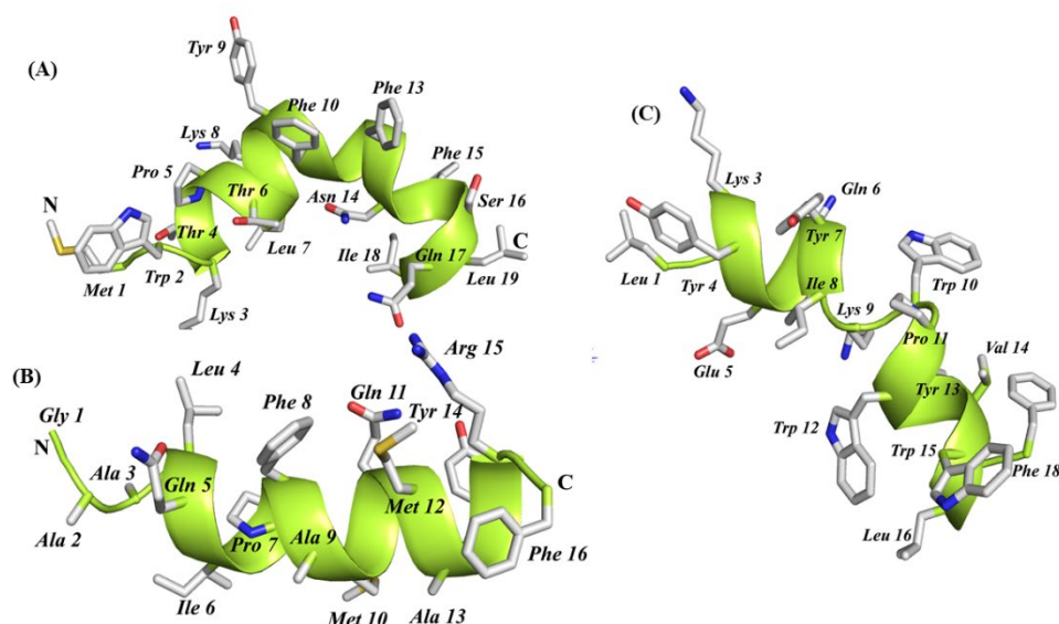
Figure 8. Ribbon representation of the structures of the fusion peptides, determined in DPC micelle, of SARS-CoV-1 (A) FP (B) IFP2 (B) and (C) PTM. Figure has been prepared using PyMOL using pdb coordinates of FPs [96].
