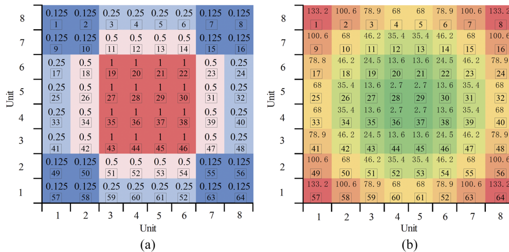
FIG. 6. (a) Amplitude (linear value) and (b) phase (°) distribution of the transmitting array.
