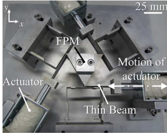
Figure 2.25: Large-workspace 3-DOF ( X - Y - \theta_z ) CPMs with optimized stiffness and dynamic properties [74].
