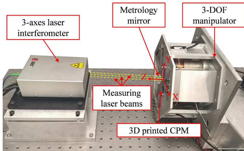
Figure 4.15: Experimental setup for measuring the positioning resolution of the manipulator.
