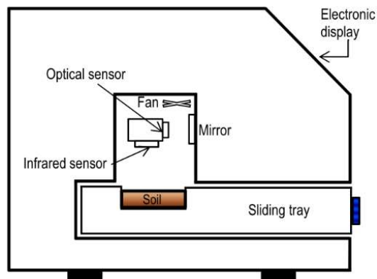
Figure 14: Schematic diagram of dew point method apparatus
