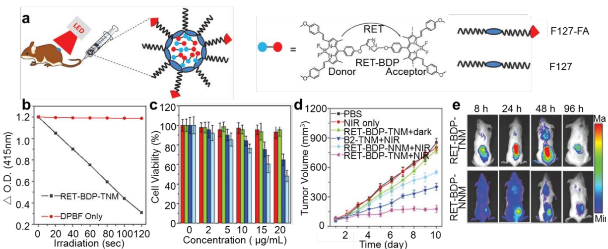
Figure 5. RET-photosensitizer nanomicelles (RET-BDP-TNM) for NIRF and guided PDT. (a) Schematic illustration for PDT of RET-BDP-TNM and the molecular structure of RET-BDP. (b) ^1\text{O}_2 generation of RET-BDP-TNM under a NIR light irradiation ( 10 \text{ mW/cm}^2 ). (c) Relative viability and photocytotoxicity of 4T1 cells incubated with different concentrations of RET-BDP-TNM and B2-TNM. (d) Change in tumor size in different groups after treatment. (e) In vivo
