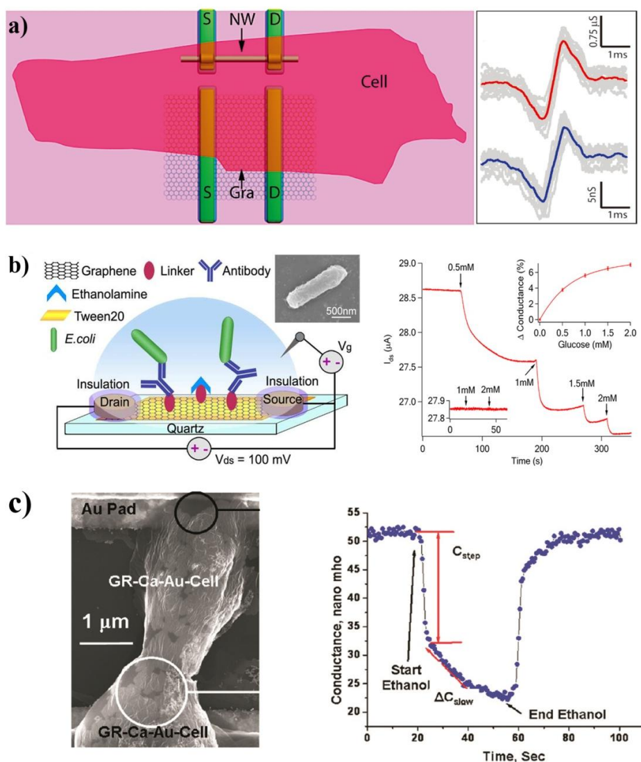
Figure 7. Electronic graphene sensors for cellular detection. (a) Detection of cellular bioelectricity. Left: Representation of a cardiomyocyte cell interfaced to a graphene-FET and a silicon nanowire-FET device; Right: thirteen electrical signals (gray traces) from the graphene-FET (upper data) and the silicon nanowire-FET (lower data) devices in response to the spontaneous action potentials produced by the cardiomyocyte. The peaks were aligned in time and the average was plotted in red and blue, respectively. Adapted from ref 235. Copyright 2010 American Chemical Society. (b) Detecting bacteria and their metabolic activity. Left: Illustration of anti- E. coli antibody functionalized graphene-FET for detection of E. coli . Inset: Scanning electron microscopy (SEM) image of an E. coli on antibody functionalized CVD-graphene. Right: Real-time current recording ( V_{ds}=100 mV and V_g=0 V) of a
