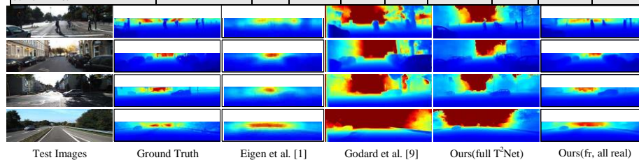
Fig.6. Qualitative results on KITTI, Eigen split [4]. The ground truth depths in the original dataset were very sparse and have been interpolated for visualization. We converted the disparity maps provided in [10] to depth maps.
