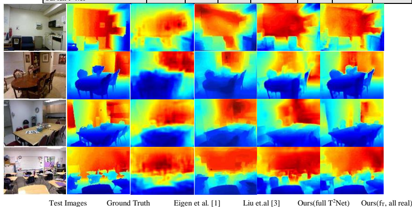
Fig.4. Qualitative results on NYUDv2. All results are shown as relative depth maps (red=far, blue=close). See text for details.
