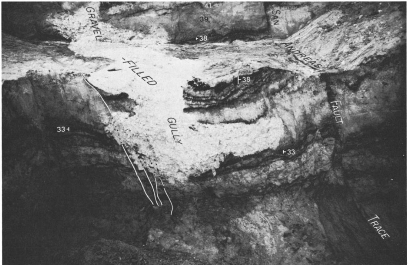
Fig. 10. Photograph of a gully that was cut into the sediments and partially filled with gravel before event R. View is southeastward. Fault on right intersects gully farther to northwest (in front of plane of paper) and offsets it 7.1 m (see Plate 3, panels 9 and 12). Fault zone on left is cut by gully and clearly antedates it. Along part of its course this gully is a subterranean pipe, eroded into units 34–50 but not breaking the ground surface that existed at the time of formation of the feature.
