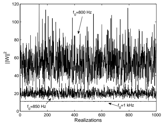
Fig. 3. \|\hat{\mathbf{W}}\|^2 versus random realizations of \mathbf{U} , where \hat{N}_T = 11 , and the minimum values of \|\hat{\mathbf{W}}\|^2 are 14.9353, 12.1387, and 10.6882 for f_0 = 800, 850, and 1 kHz, respectively.
