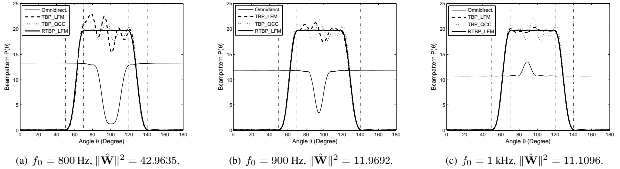
Fig. 2. Designed transmit beampatterns using standard and robust techniques, where \hat{N}_T = 11 , and \mathbf{U} = \mathbf{U}_0 = \mathbf{I} .
