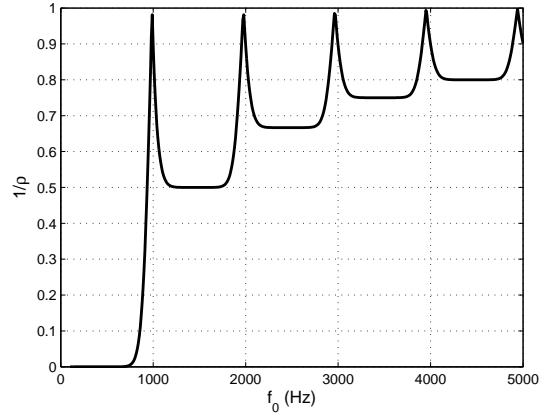
Fig. 1. 1/\rho versus f_0 , where B = 100 kHz, and T = 1 ms.
