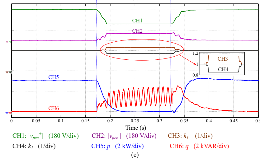
Fig. 10. Experimental results: Sag II: (a) Three-phase voltage and currents, (b) dc-link voltage, PV string voltage, current and power and (c) positive- and negative-sequence voltages, k_1 , k_2 and injected active/reactive power.
