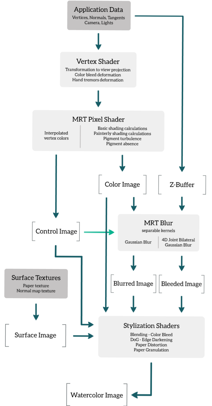
Figure 4: System schematic of the rendering pipeline. Dark gray elements represent the input data, gray elements represent the different processing stages and the bracketed elements represent the computed images in the frame buffers.
