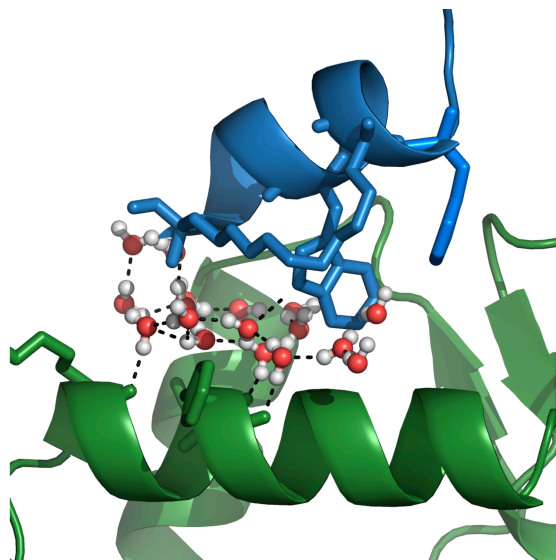
Figure 6. An intricate water structure formed between the staple and MDM2 for Stapled. Water molecules are shown in ball and sticks (red for oxygen and white for hydrogen) while the key hydrophobic residues of Stapled (F19, W23 and L26 based on full p53 sequence) and the staple are shown in sticks. Residues on MDM2 that interact with the water network are also highlighted in stick format.
