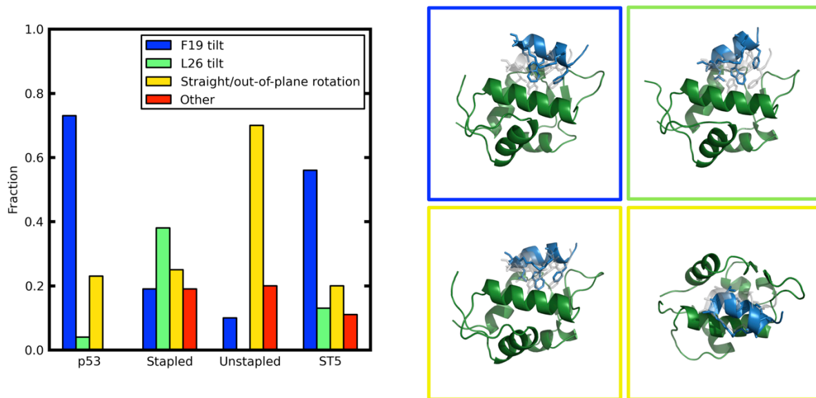
Figure 3. Binding mechanisms for p53, Stapled, Unstapled and ST5. p53 preferentially binds MDM2 by tilting in the F19 direction. The presence of the staple changes the binding mechanism of Stapled compared to p53, as the increased helix stability enables the peptide to tilt or orient to bind MDM2 more readily. Differences observed in MDM2-binding for Unstapled compared to p53 suggest that the sequence and length of the peptide likely affects its binding mechanism too.
