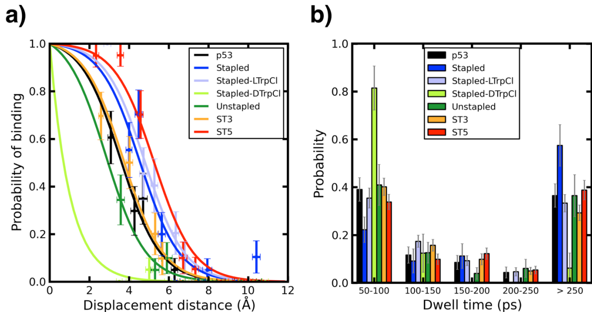
Figure 2. (a) Probability that the different peptides rebind (see Materials and Methods for definition) to MDM2 as a function of displacement distance (taken as initial backbone RMSD after equilibration). For visualization, sigmoidal fits to the data are also shown. ST5, Stapled-LTrpCl and Stapled rebind with higher propensity than p53 while ST3 and Unstapled rebind as a function of displacement distance similar to p53. Stapled-DTrpCl is essentially unable to rebind when displaced. Errorbars are obtained from bootstrapping (see Materials and Methods). (b) The time (“dwell time”) the peptide fluctuates within the bound state ( \leq 2 Å peptide backbone RMSD). Statistics were gathered from all independent simulations and normalized by number of “bound windows” (see Materials and Methods).
