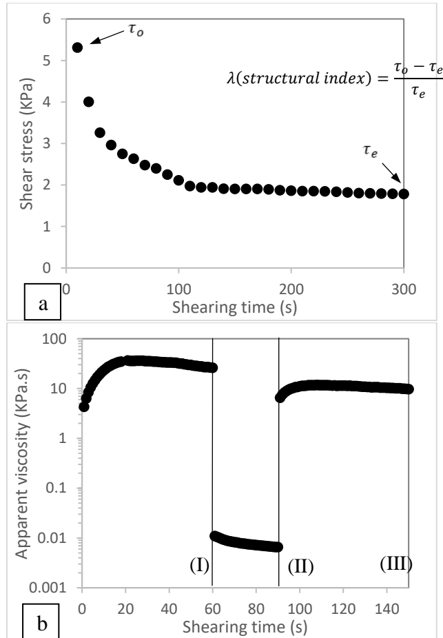
Figure 1. Thixotropy behaviour of 3D printed concrete (a) structural breakdown (b) structural recovery.
