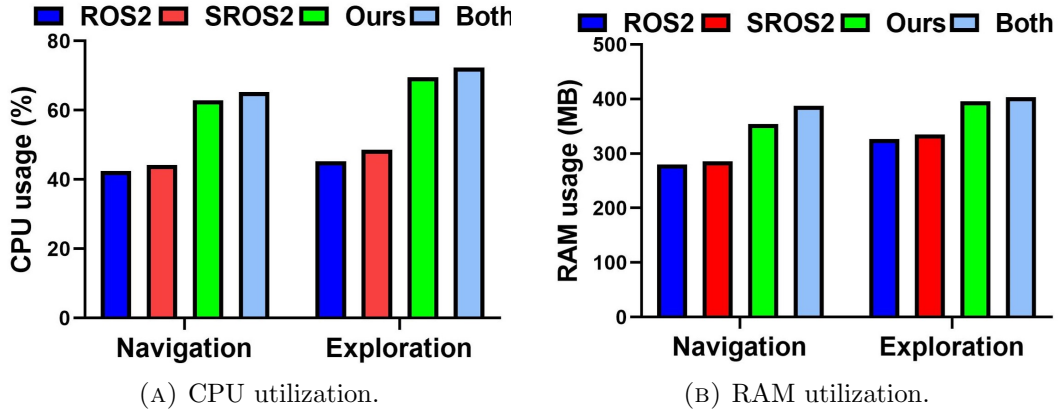
FIGURE 4.12: Resource consumption of four implementations.
