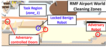
(A) Exploiting V1 to terminate the workload (airport world).
