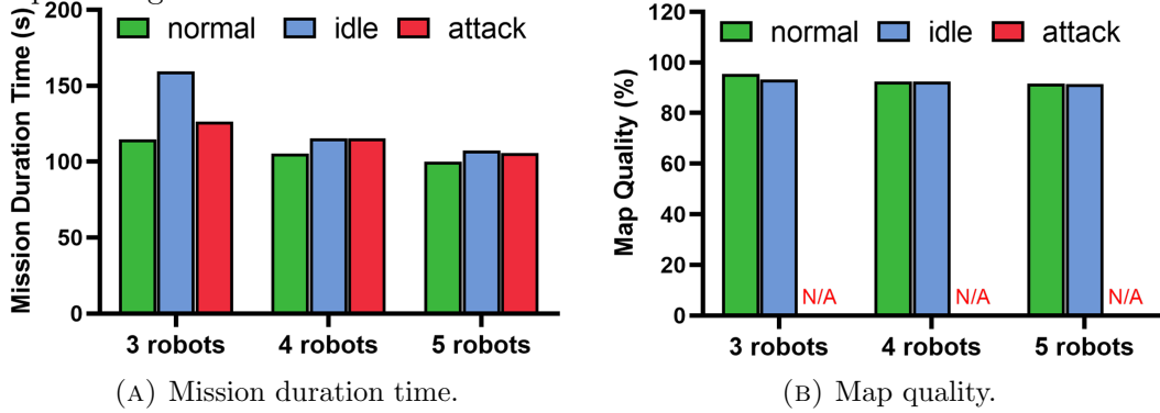
FIGURE 3.16: Map merging poisoning attack against W3 .
