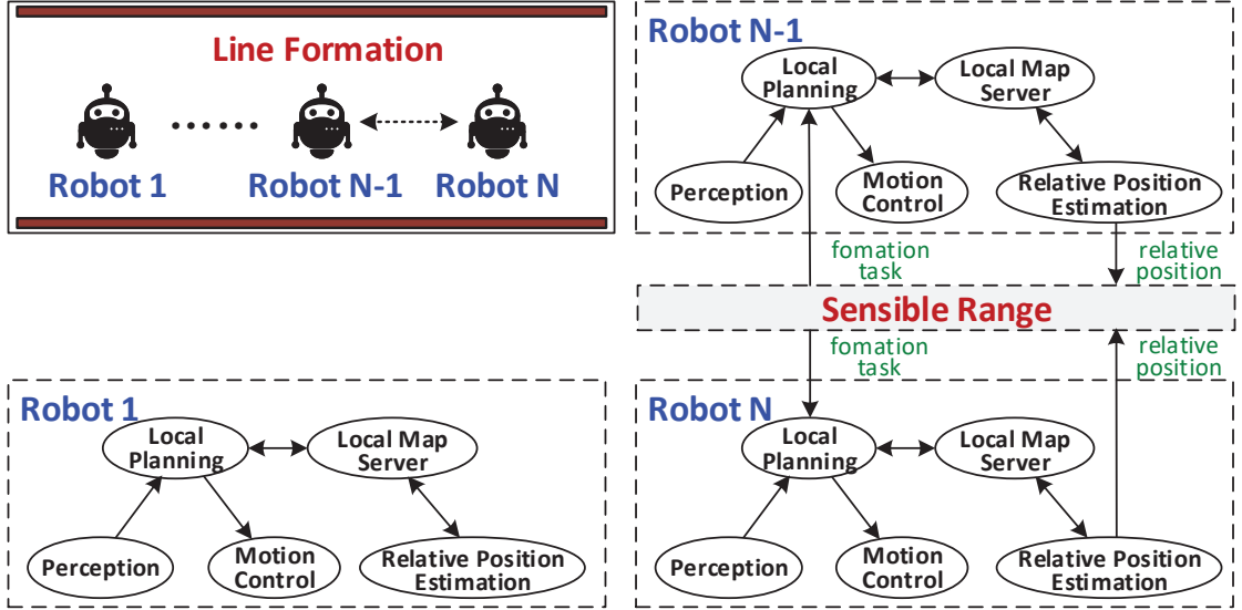
FIGURE 3.8: Workflow of W5
