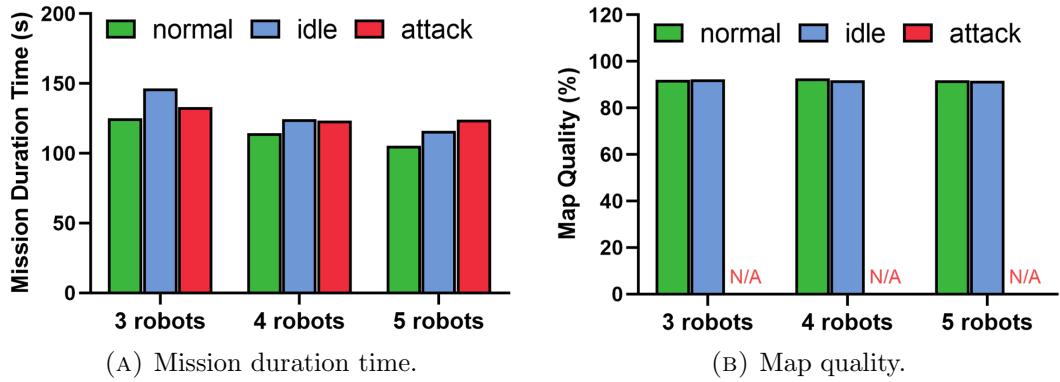
FIGURE 3.18: Blocking group merging attack against W4 .
