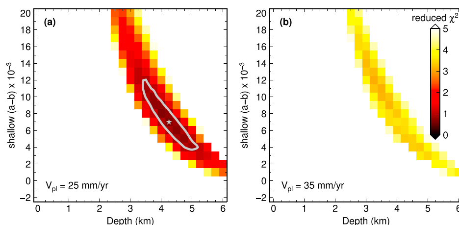
Figure 9. Reduced \chi^2 misfit for the three data sets combined. The case of a (a) 25 mm/yr driving rate and (b) 35 mm/yr driving rate. Starred model corresponds to a velocity-strengthening layer depth of 4.25 km with (a - b) = 0.007 (shown in Figure 6b).
