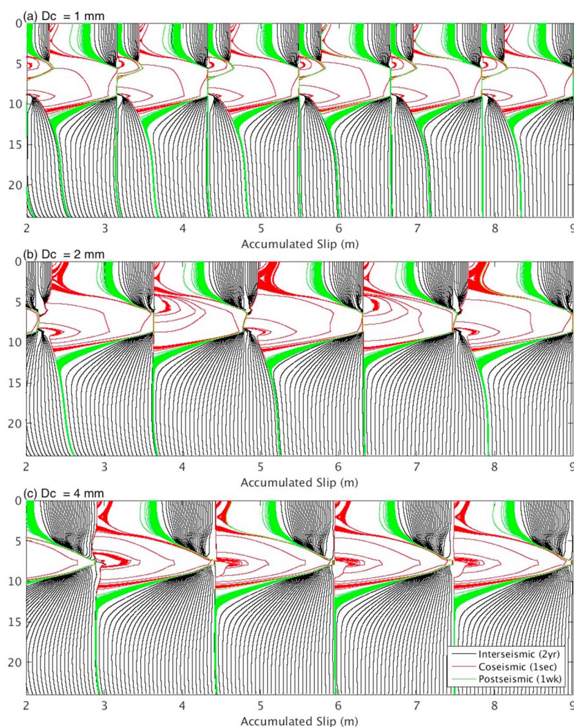
Figure 10. Models showing the effect of reducing the value of the slip-weakening distance D_c . When D_c is smaller than 4 mm as in (a) and (b), a new periodic sequence of two different-sized earthquakes develops. Models considered in the text assume D_c = 4 mm, as in (c). Other parameters correspond to the gray star in Figure 9.
