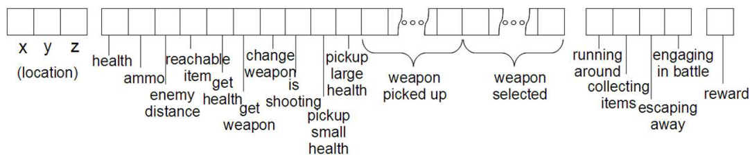
Figure 4.6: The input vectors of state, action, and reward to RLBot and RLBot++ in UT
