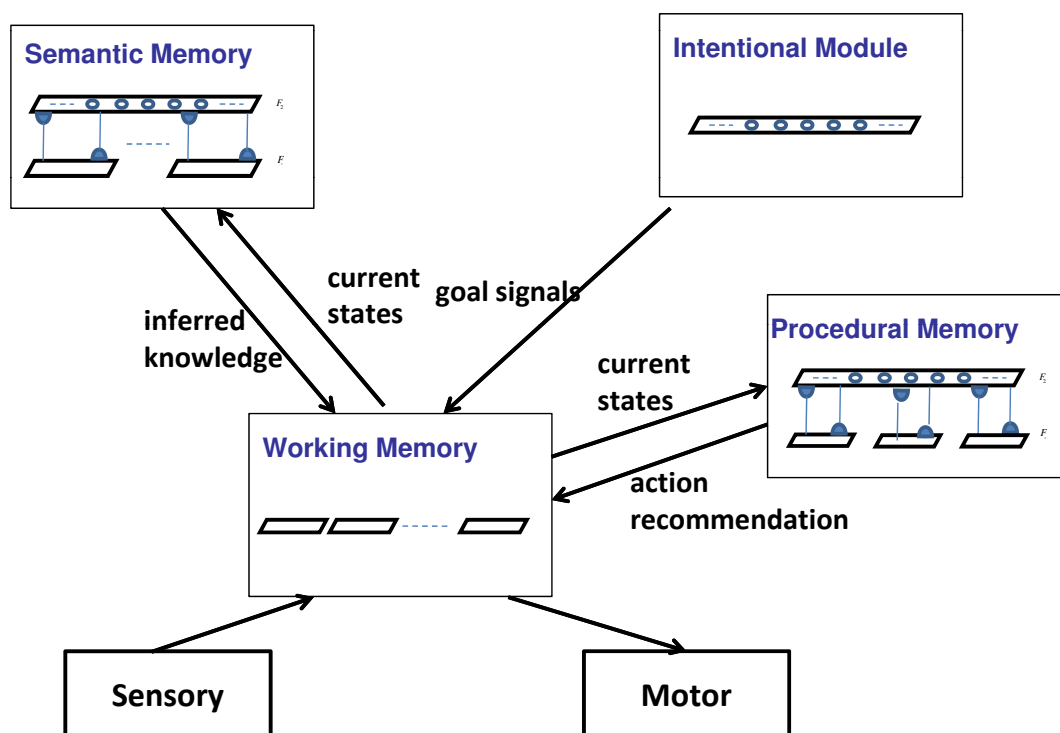
Figure 5.1: The proposed framework of the dual-memory cognitive model.
