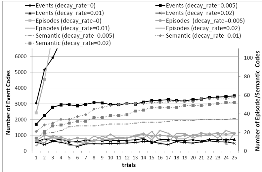
Figure 4.7: Memory usage for events, episodes, and transferred semantic knowledge with different forgetting decay rate during the game play
