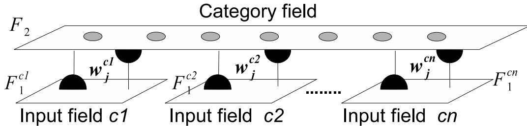
Figure 5.2: The fusion ART Architecture
