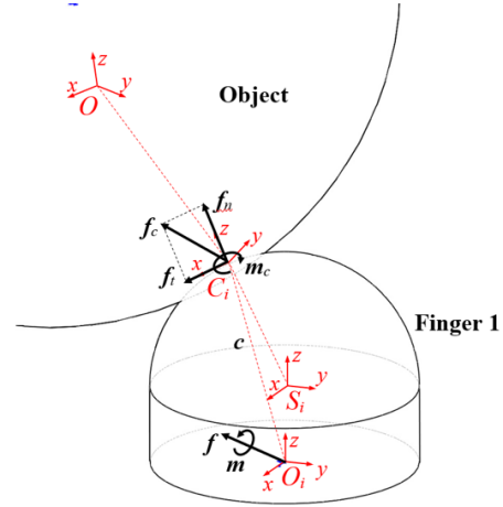
Fig.2. Force equilibrium of contact model. \{O_i - xyz\} , \{S_i - xyz\} , \{C_i - xyz\} denote the sensor frame, the fingertip frame, the contact frame and the object frame, respectively; f_c and m_c are the contact force and moment, respectively; f_n and f_t represent the normal and tangential forces in \{C_i - xyz\} . c is the position vector between \{O_i - xyz\} and \{C_i - xyz\} .
