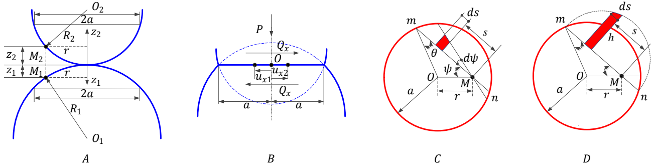
Fig. 6. Soft contact. At the beginning, without the load, two bodies just contact at one point(A). There are two points M_1 and M_2 being r away from the common normal and being z_1, z_2 away from the tangential plane between two bodies, respectively. When a force P is applied to loading along the normal, the local deformation results in a circular contact surface with the radius a around the contact point(B). Due to the local deformation, M_1 and
