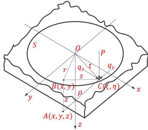
Fig. 5. The model of the elastic half-space.
