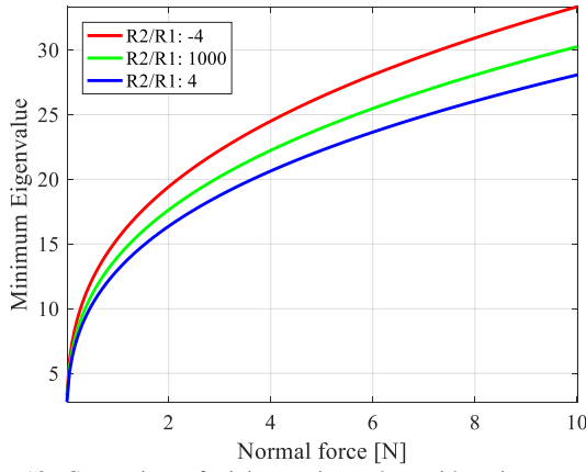
Fig. 12. Comparison of minimum eigenvalues with various contact local curvatures.
