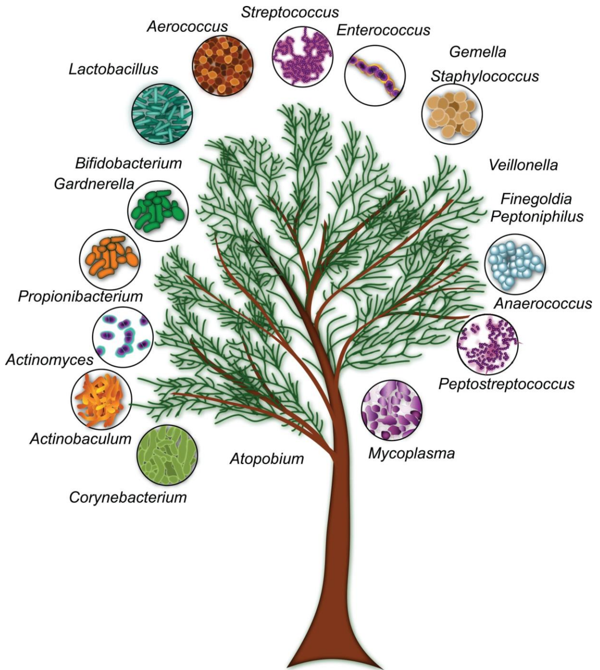
Figure 2. Gram-positive inhabitants and pathogens of the human urinary tract
