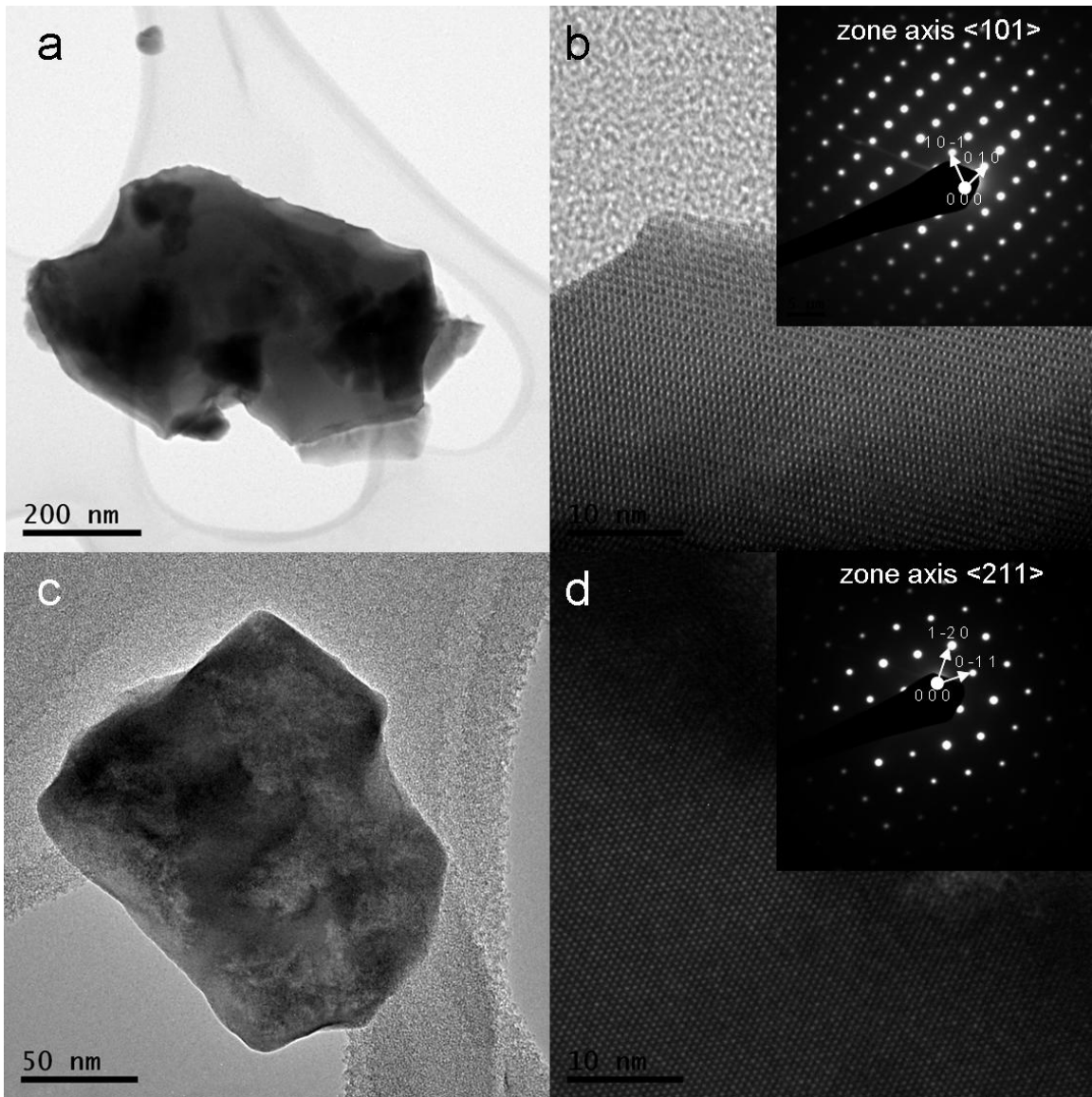
Fig. 7 TEM images (low-magnification and high-resolution) and diffraction patterns for nominal (a) & (b): [\text{La}_8\text{Sr}_2][\text{Ge}_6]\text{O}_{26} , (c) & (d): [\text{La}_8\text{Sr}_2][\text{Ge}_{5.5}\text{V}_{0.5}]\text{O}_{26.25} .
