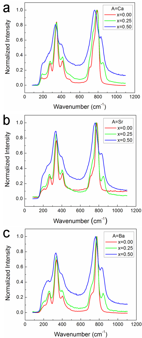
Fig. 8 Raman spectra of normalised intensities for (a) \text{La}_8\text{Ca}_2\text{Ge}_{6-x}\text{V}_x\text{O}_{26+x/2} , (b) \text{La}_8\text{Sr}_2\text{Ge}_{6-x}\text{V}_x\text{O}_{26+x/2} , (c) \text{La}_8\text{Ba}_2\text{Ge}_{6-x}\text{V}_x\text{O}_{26+x/2} series with nominal x = 0, 0.25 , and 0.5 , measured at room temperature.
