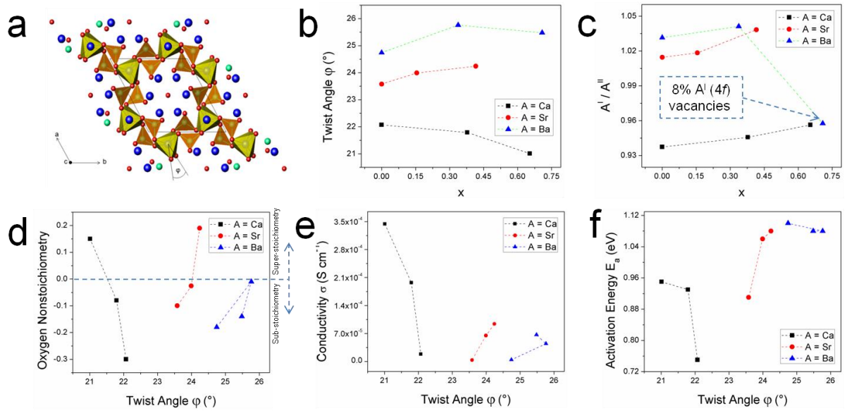
Fig. 4 Twist angle (a) Polyhedral representation of the refined \text{La}_{7.99}\text{Sr}_2\text{Ge}_{5.58}\text{V}_{0.42}\text{O}_{26.20} structure with metaprism twisting ( \phi ) labelled, face-sharing \text{A}^{\text{I}}\text{O}_6 metaprisms (yellow) are corner connected to \text{BO}_4 tetrahedra (orange) forming the framework, which surrounds the tunnel \text{A}^{\text{II}} atoms (blue), (b) Plot of twist angles with respect to x , (c) Plot of \text{A}^{\text{I}}/\text{A}^{\text{II}} atomic size ratio with respect to x , (d) Plot of oxygen nonstoichiometry with respect to \phi , (e) Plot of ionic conductivity with respect to \phi , (f) Plot of activation energy with respect to \phi for \text{La}_8\text{AE}_2\text{Ge}_{6-x}\text{V}_x\text{O}_{26+x/2} ( \text{AE} = \text{Ca}, \text{Sr}, \text{Ba} ).
