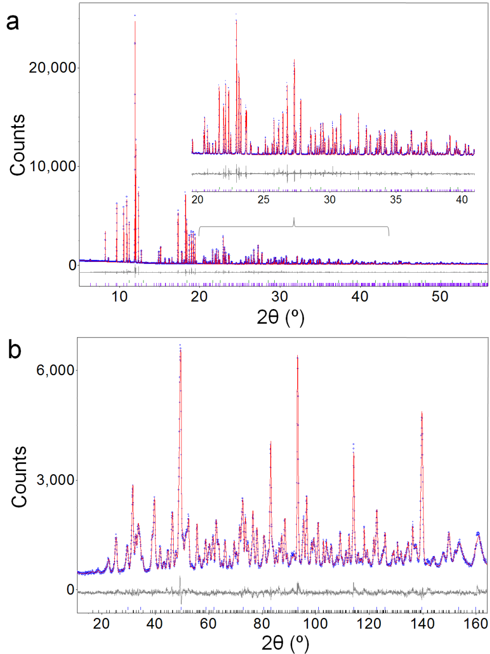
Fig. 3 Rietveld plots of the (a) synchrotron and (b) neutron powder diffraction data of nominal \text{La}_8\text{Sr}_2\text{Ge}_{5.5}\text{V}_{0.5}\text{O}_{26.25} collected at room temperature. The observed intensity is shown by dots, with the solid line representing the calculated intensity. Differences between observed and calculated intensities are plotted beneath. Vertical markers indicate the Bragg reflections of \text{CaF}_2 standard (top) and apatite (bottom).
