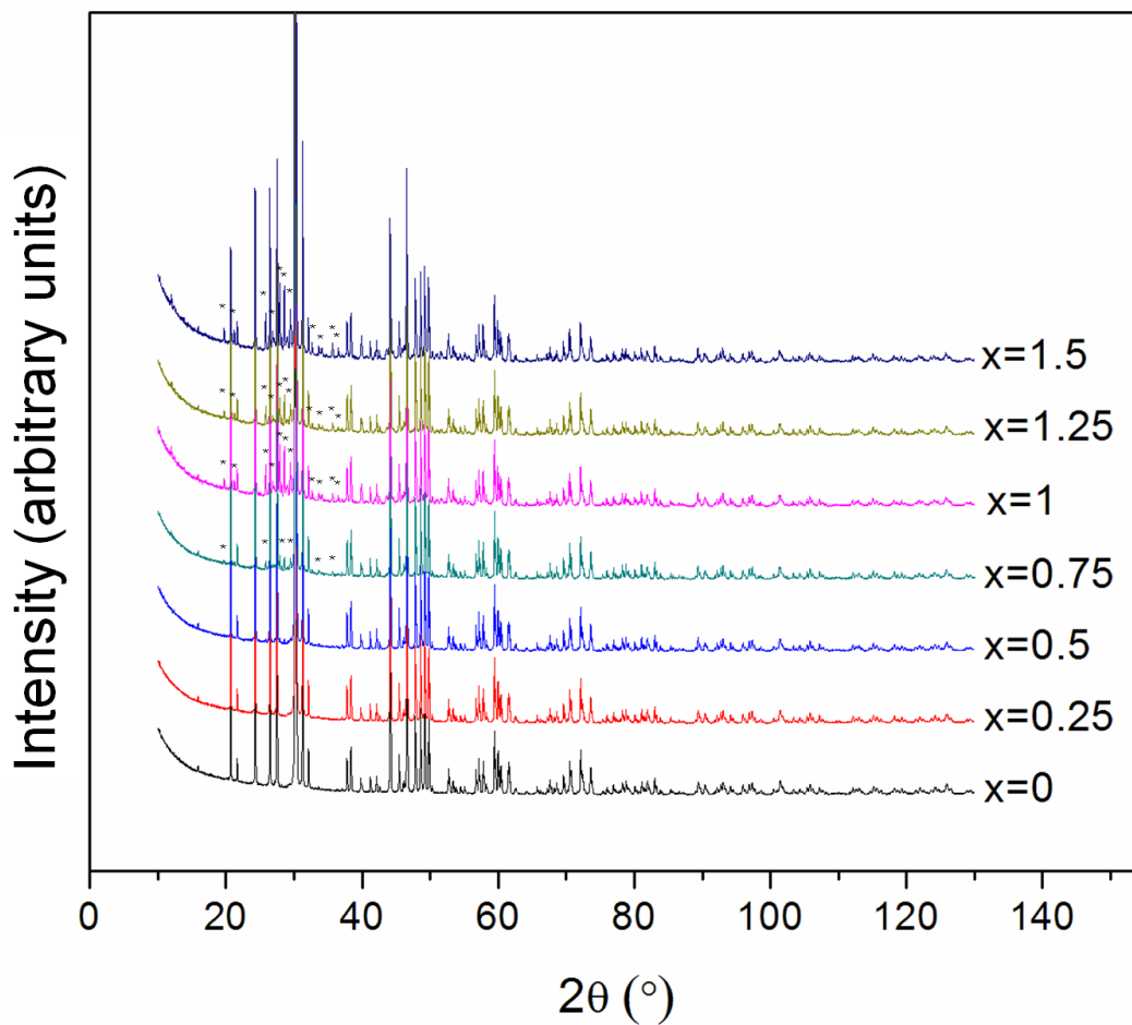
Fig. 1 PXRD data for [\text{La}_8\text{Sr}_2][\text{Ge}_{6-x}\text{V}_x]\text{O}_{26+x/2} series with x=0, 0.25, 0.5, 0.75, 1, 1.25, and 1.5 synthesised with two calcination cycles at 1300 and 1350 ^\circ\text{C} for 16 hours separately. Under these preparative conditions the solid solution limit is x = 0.5 . For x > 0.5 , peaks from secondary phases are labelled with *.
