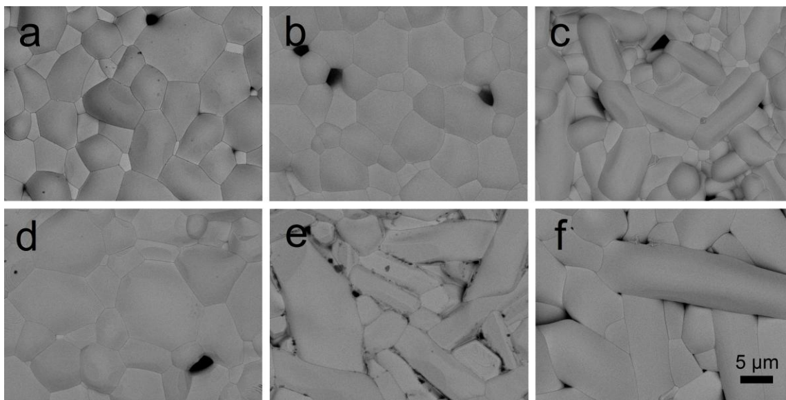
Fig. 5 Low angle backscattered electron micrographs (5.0kV) for [\text{La}_8\text{AE}_2][\text{Ge}_{6-x}\text{V}_x]\text{O}_{26+x/2} series with (a) \text{AE} = \text{Ca} , x = 0 ; (b) \text{AE} = \text{Sr} , x = 0 ; (c) \text{AE} = \text{Ba} , x = 0 ; (d) \text{AE} = \text{Ca} , x = 0.5 ; (e) \text{AE} = \text{Sr} , x = 0.5 ; (f) \text{AE} = \text{Ba} , x = 0.5 .
