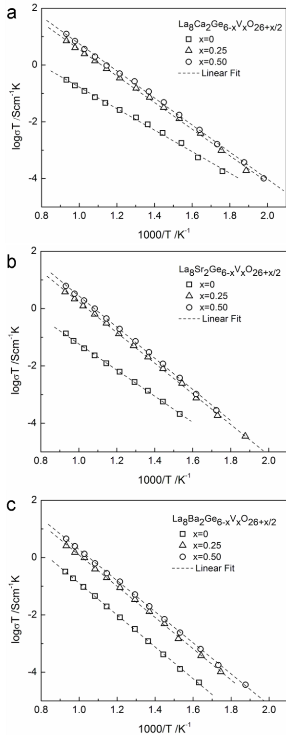
Fig. 9 Variation of conductivities with temperatures for (a) \text{La}_8\text{Ca}_2\text{Ge}_{6-x}\text{V}_x\text{O}_{26+x/2} , (b) \text{La}_8\text{Sr}_2\text{Ge}_{6-x}\text{V}_x\text{O}_{26+x/2} , (c) \text{La}_8\text{Ba}_2\text{Ge}_{6-x}\text{V}_x\text{O}_{26+x/2} series with nominal x = 0, 0.25, and 0.5 .
