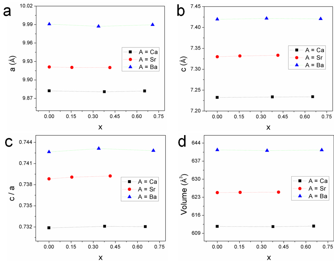
Fig. 2 Refined lattice parameters from synchrotron powder X-ray diffraction data for \text{La}_8\text{AE}_2\text{Ge}_{6-x}\text{V}_x\text{O}_{26+x/2} ( \text{AE} = \text{Ca}, \text{Sr}, \text{Ba} ) (a) a , (b) c , (c) c/a , (d) unit cell volume. The x -values are those derived from Rietveld analysis.
