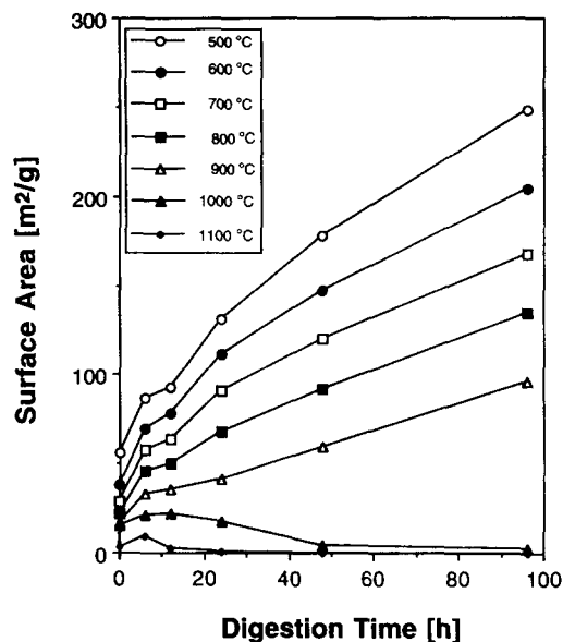
Fig. 2. Effect of time of digestion at 100°C on the surface area of zirconia. Heat treatment: 12 h at each temperature.
