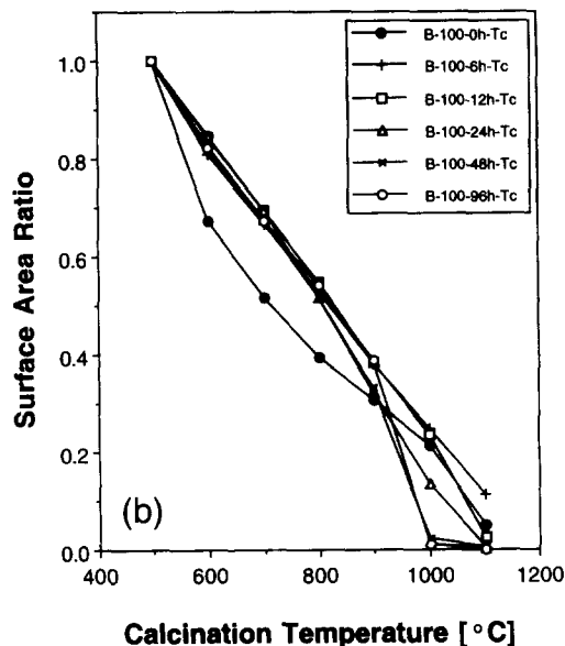
Fig. 4. (a) Relative surface area ( S_T/S_{500^\circ\text{C}} ) versus calcination temperature for zirconia prepared using the acidic, basic and lanthanum-doped methods. Dotted lines are for zirconia prepared from precursors which had been aged at 30^\circ\text{C} while unbroken lines are from precursors which had been digested at 100^\circ\text{C} . (b) Relative surface area ( S_T/S_{500^\circ\text{C}} ) versus calcination temperature for zirconia prepared from digestion of the precursor for different lengths of time at 100^\circ\text{C} .
