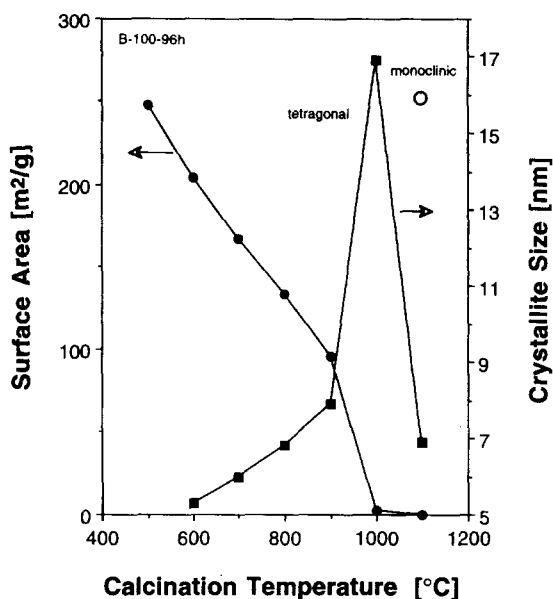
Fig. 5. Crystallite size of the tetragonal and monoclinic phase versus calcination temperature.
