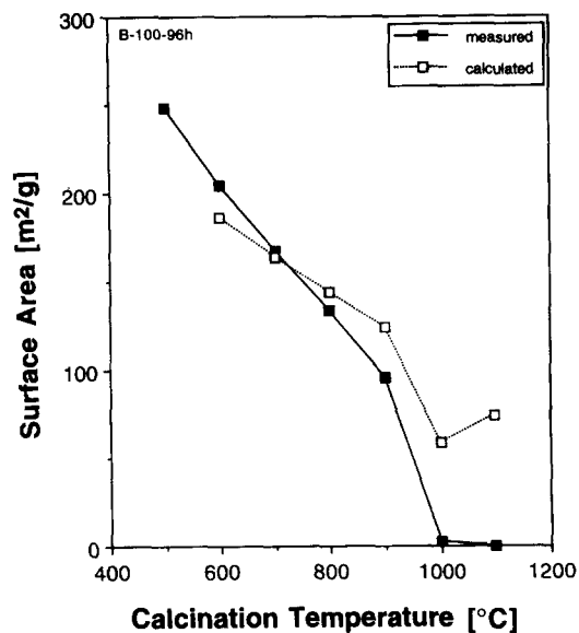
Fig. 6. Comparison of measured BET surface area with the surface area calculated for spherical particles based on the dimensions derived from x-ray line broadening.
