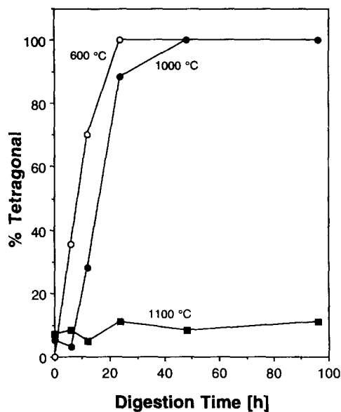
Fig. 3. Amount of tetragonal phase as a function of digestion time for zirconia, B-100-96h, heat treated to 600°C, 1000°C and 1100°C.
