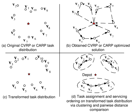
Fig. 6. An illustration example of how the success of task assignment and task servicing ordering in the optimal solution s are archived by a transformation.
