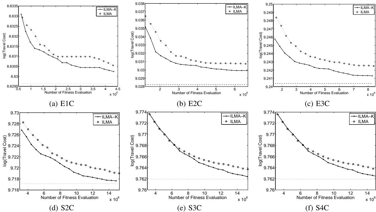
Fig. 9. Averaged search convergence graphs of ILMA and ILMA-K on representative CARP benchmark instances. Y-axis: \log(\text{Travel Cost}) , X-axis: Number of Fitness Evaluation. (The dashed line at the bottom of each figure denotes the lower bound or best known solution of the respective benchmark reported in the literature.)
