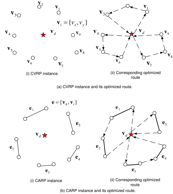
Fig. 1. An illustration of CVRP and CARP instances and their respective optimized solutions.
