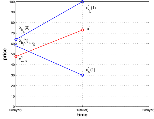
Fig. 4 Backward induction construction with the same setting as in Fig. ?? except RP_l = 30 .
