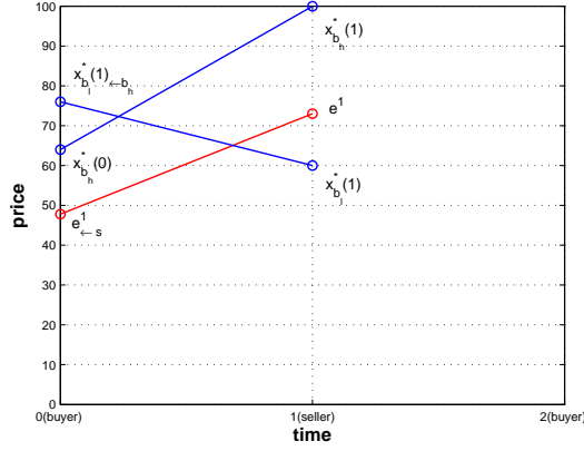
Fig. 3 Backward induction construction with T = 2 , \iota(T) = \mathbf{b} , RP_h = 100 , \omega_{\mathbf{b}_h}^0 = 0.7 , RP_l = 60 , \omega_{\mathbf{b}_l}^0 = 0.3 , RP_s = 10 , \delta_s = \delta_b = 0.6 .
