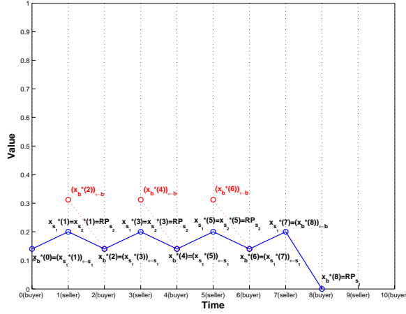
Fig. 1 Backward induction construction with RP_b = 1 , RP_{s_1} = 0 , RP_{s_2} = 0.2 , \delta_b = 0.8 , \delta_{s_1} = 0.7 , \delta_{s_2} = 0.8 , T_b = 10 , T_{s_1} = 11 , T_{s_2} = 7 ; at each time point t the optimal offer x_a^*(t) that \iota(t) can make is marked; the dashed lines are sellers' optimal offer if there is only one seller.
