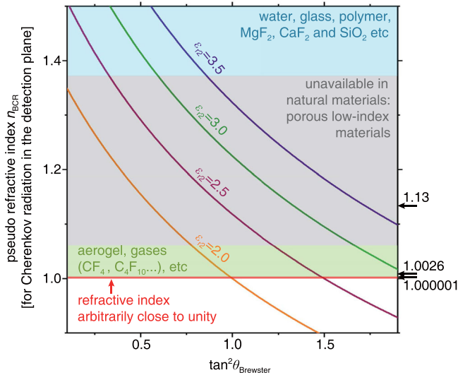
Fig. 3 Engineering the pseudo refractive index n_{BCR} for Brewster-Cherenkov detectors, achieving parameter regimes that do not exist in natural materials. For the transmitted Cherenkov radiation in the detection plane, its wavevector component parallel to the detection plane has k_{BCR} = n_{BCR} \omega/c , where n_{BCR} = \sqrt{\frac{\epsilon_1 \epsilon_2}{\epsilon_1 + \epsilon_2}} . Here we plot n_{BCR} as a function of the Brewster angle \theta_{Brewster} under different values of \epsilon_{r2} , where \tan \theta_{Brewster} = \sqrt{\epsilon_{r2}/\epsilon_{r1}} .
