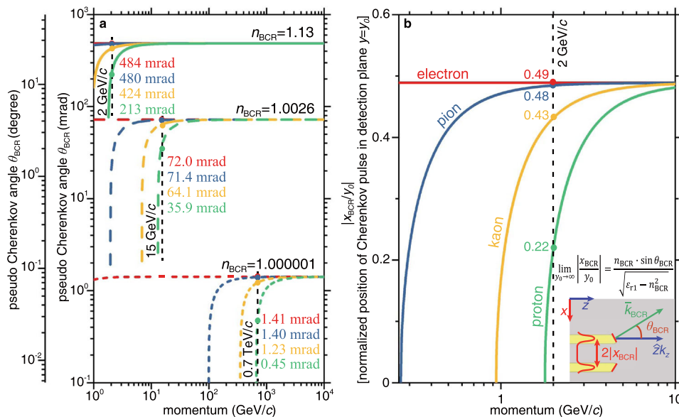
Fig. 4 Performance of Brewster-Cherenkov detectors in the identification of high-energy particles. a Pseudo Brewster-Cherenkov angle \theta_{BCR} versus particle momentum. This figure is plotted according to the generalized Frank-Tamm formula \cos \theta_{BCR} = \frac{c}{n_{BCR} v} , by transforming the particle velocity to the momentum. The values of pseudo Brewster-Cherenkov angles for four elementary particles, namely electron (red), pion (blue), kaon (yellow), and proton (green), with a momentum of 2, 15, or 700 GeV/c are given in the plot. b Normalized peak-intensity position |x_{BCR}/y_0| of the transmitted Cherenkov radiation in the detection plane versus particle momentum. The measurement of |x_{BCR}/y_0| provides the information of \theta_{BCR} and further the particle velocity. In (b), y_0 = 2.3 mm and n_{BCR} = 1.13 .
