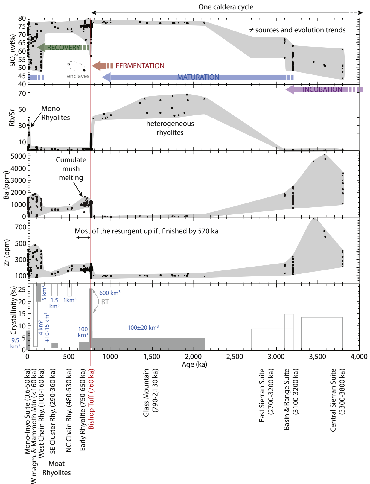
Fig. 3. Temporal evolution of magma compositions (bulk rock SiO 2 , Rb/Sr, Ba, and Zr contents) and crystal content at Long Valley caldera. Notice the particularly high Ba and Zr contents in the Early Rhyolite, that we interpret as post-Bishop Tuff cumulate mush melting. When known, erupted volumes for the various eruptive episodes are labeled in blue next to the average crystal content of magmas from the same episode. Purple, blue, red and green arrows indicate the timings of the incubation, maturation, fermentation, and recovery phases, respectively. Data is from Metz and Mahood (1991), Bailey (2004), Hildreth and Wilson (2007), Van Kooten (1980), Hildreth (2017), Heumann and Davies (1997), Sampson and Cameron (1987), and Kelleher and Cameron (1990). Duration of the resurgent uplift is from Hildreth et al. (2017). LBT = Late Bishop Tuff. (For interpretation of the references to colour in this figure legend, the reader is referred to the web version of this article.)
