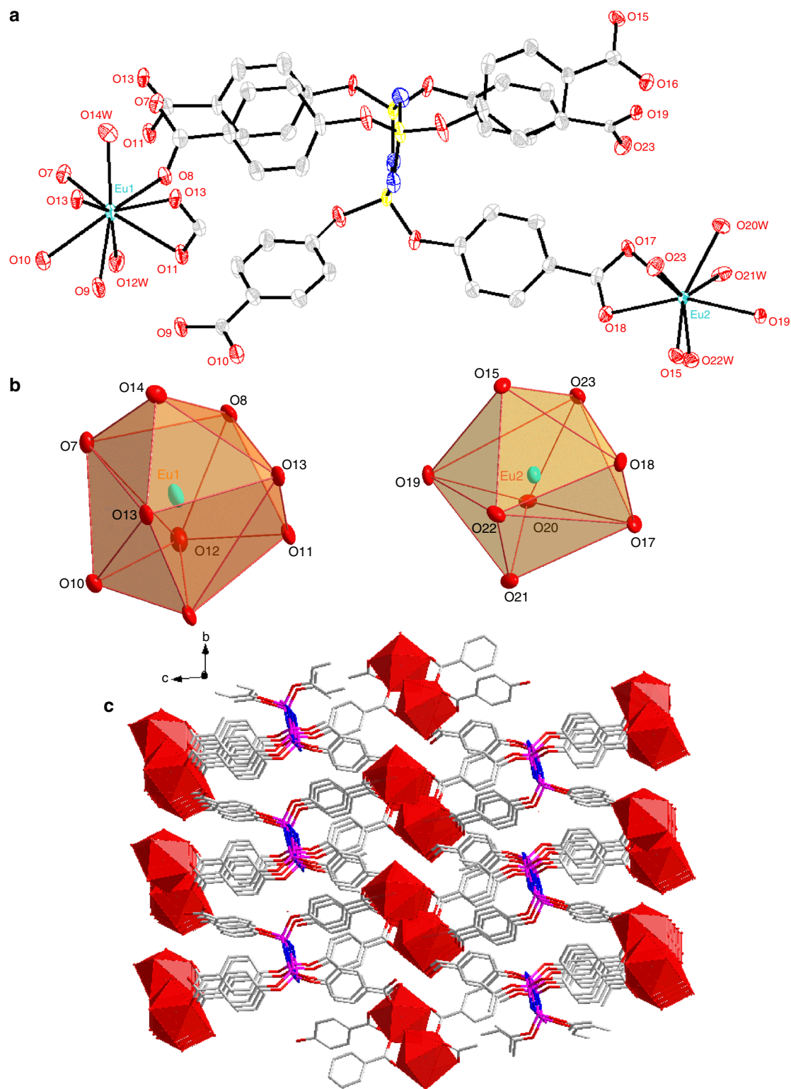
Fig. 1 Crystal structure of Eu-CTP-COOH. a Coordination environment around Eu 3+ ion (50% ellipsoids) with hydrogen atoms being omitted for clarity. b Tri-capped triangular prismatic and bi-capped triangular prismatic geometry of Eu1 and Eu2 in Eu-CTP-COOH, respectively. c Packing framework of Eu-CTP-COOH, where Eu 3+ is represented as a polyhedron
