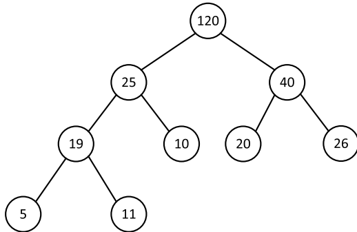
Fig. 11. Binary max heap data structure.
