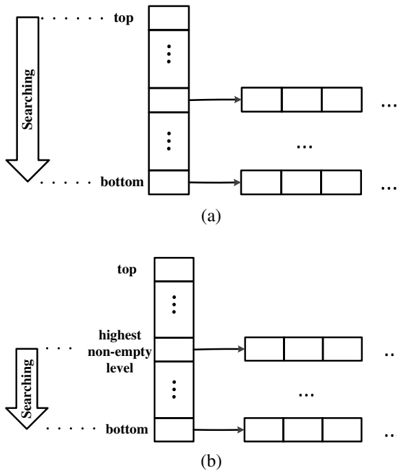
Fig. 2. Searching the highest nonempty level. (a) Refreshed searching and (b) resumed searching.
