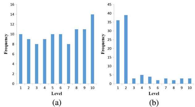
Fig. 9. (a) Histogram of quality distribution with adaptive mapping and (b) histogram of quality distribution with fixed mapping.
