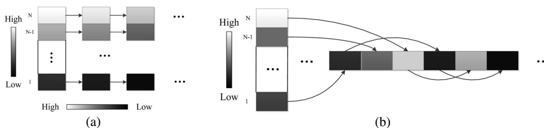
Fig. 1. (a) Indexed linked list and (b) I2L2.
