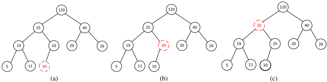
Fig. 12. Operations of inserting a new element. (a) The new element is inserted to the end of the heap. (b) and (c) Subsequent steps of moving the new element to the proper position.
