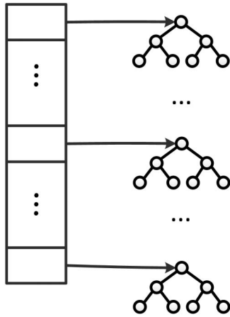
Fig. 14. Structure of I2L2-H.
