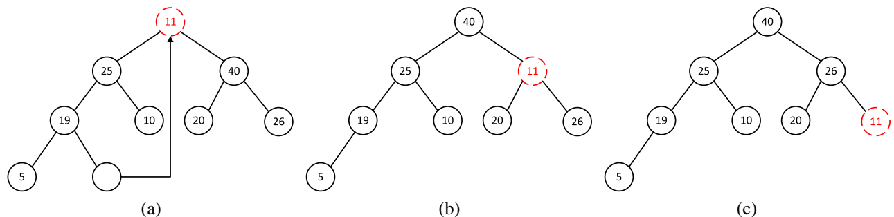
Fig. 13. Operations of restoring heap order after deleting the root element. (a) Replace the root with the last element. (b) and (c) Subsequent steps of restoring the order of the heap.
