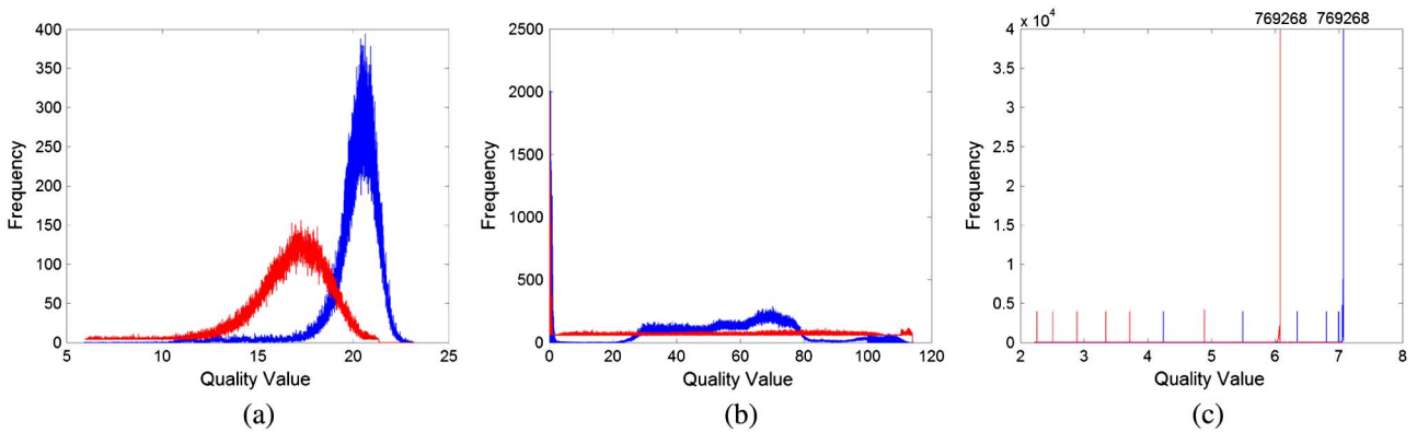
Fig. 10. Quality distribution curves comparison between the fixed and adaptive mapping. The blue curve represents the fixed mapping, and the red curve is the adaptive mapping. (a) Peaks, (b) coffee cup lid, and (c) toy duck.
