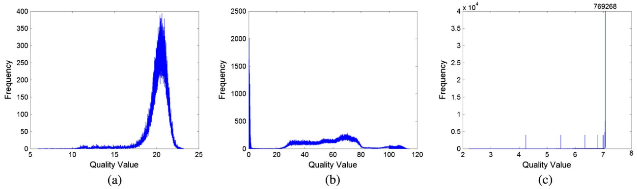
Fig. 6. Quality distribution curves. (a) Peaks, (b) coffee cup lid, and (c) toy duck.
