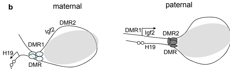
Figure 1-3 Schematic representation of epigenetic regulation at Igf2/H19 imprinting domain. a. Insulator and enhancer model. The Igf2-H19 locus contains a pair of reciprocally imprinted and coordinately regulated imprinted genes controlled by an intergenic imprinting center (IC), which binds CTCF (light blue oval) when unmethylated and insulates the Igf2 fetal promoters from common downstream enhancers (yellow circles) in endoderm. In mesoderm, tissue-specific silencer DMR1 plays a role in Igf2 regulation. Tissue-specific enhancer (DMR2) upstream of the insulator regulates biallelic activity of Igf2 in parts of the brain. Adapted from (86). b. Chromatin loop model. On the maternal allele, the unmethylated H19 DMR (which is bound by CTCF and other proteins; open ovals) and Igf2 DMR1 interact, resulting in two chromatin domains, with H19 in an active domain with its enhancers (small white circles) and Igf2 in an inactive domain away from the enhancers (shaded area). On the paternal allele, the methylated H19 DMR associates with the methylated Igf2 DMR2 through putative protein factors (filled ovals), moving Igf2 into the active chromatin domain. The location of DMR2 at the end of Igf2 positions its promoters in close vicinity to the enhancers downstream of H19 . H19 is in the active domain but is silenced by DNA methylation. Drawings are not to scale. Adapted from (115).
