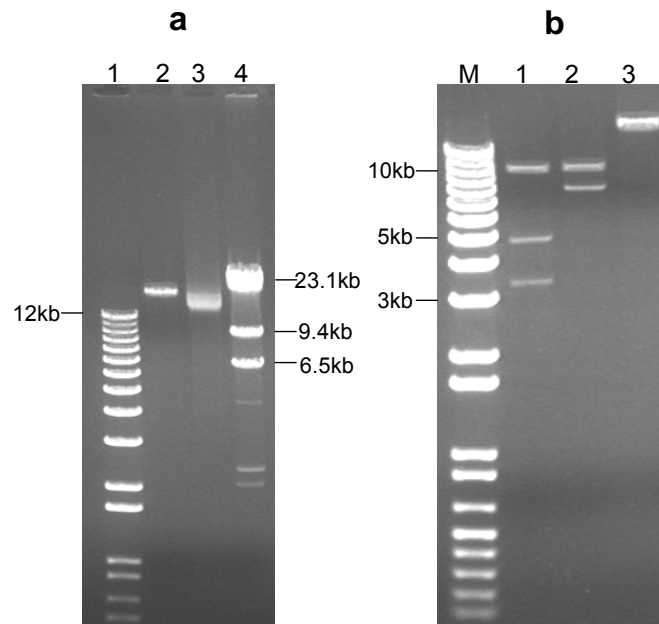
Figure 2-9 Fusion of pCMVsport \beta geoN r with pUNI-3 a. pCMVH6 was digested with NheI , lane 1: 1 kb ladder; lane 2: pCMVH6/ NheI ; lane 3: pCMVH6; lane 4: \lambda DNA/ HindIII . b. pCMVH6 further confirmation, M: 1 kb ladder; lane 1: pCMVH6/ EcoRI ; lane 2: pCMVH6/ HindIII ; lane 3: pCMVH6/ NheI .
