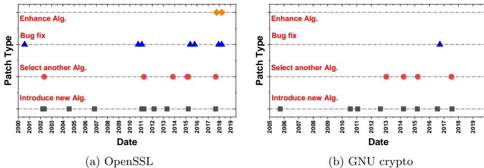
Figure 3: Countermeasure types of the two libraries
