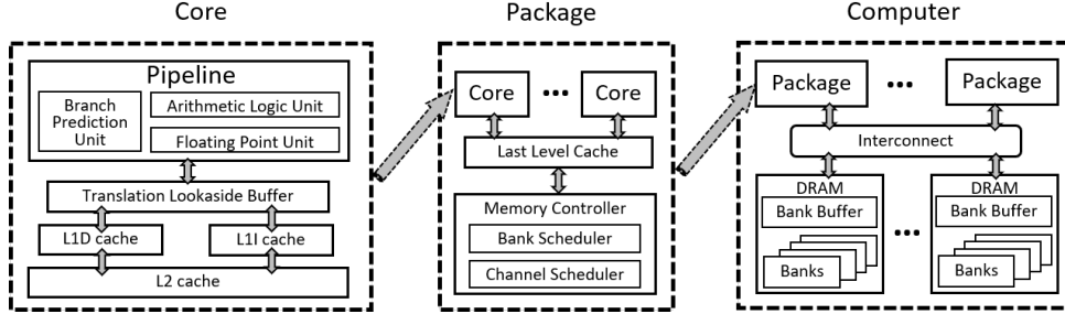
Figure 1: A Multi-core System
