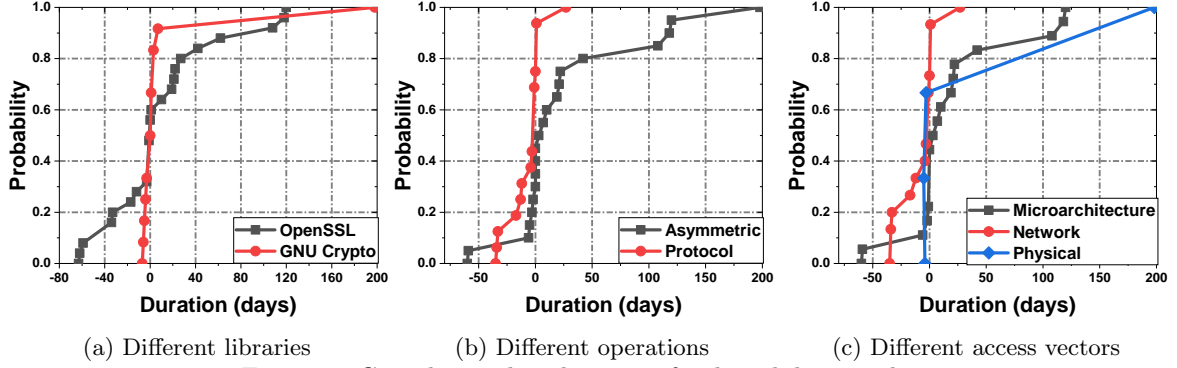
Figure 2: Cumulative distributions of vulnerability windows
