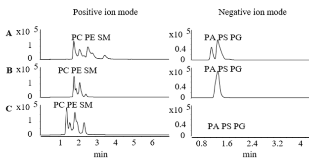
Fig. 1. Choice of column. The mobile phase A (water) and B (methanol) was used to analyze the mixed phospholipid standards. Both A and B included 5mM ammonium acetate and 0.01% formic acid. The positive ion mode detected PC, PE and SM, the negative ion mode detected PA, PG, PI and PS. A binary isocratic elution with 98% B was applied, the column was held at 45 °C and the separation was allowed at a flow rate of 0.4 mL/min. A: Agilent ZORBAX Eclipse plus C18 (2.1×100 mm, 1.8 μm); B: Agilent ZORBAX Eclipse plus C8 (2.1×150 mm, 1.8 μm); C: Phenomenex Kinetex 2.6u C18 (2.1×100 mm).
