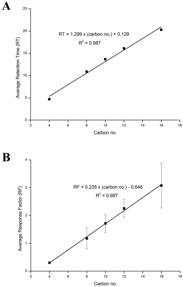
FIG. 2. Graphs depicting the linear relationship between PHA carbon number and (A) average retention time (RT), and (B) average response factor (RF). The mean values represent values from at least three independent experiments ( n \geq 3 ) and the error bars represent standard deviations.
