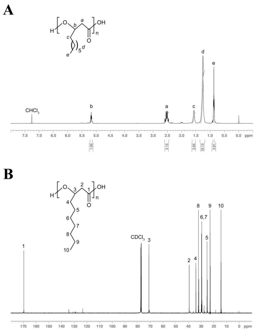
FIG. S1. (A) ^1\text{H} -NMR and (B) ^{13}\text{C} -NMR spectra of mcl-PHA polymer. The signals corresponding to hydrogen atoms in ^1\text{H} -NMR spectrum are denoted by alphabet letters while the signals corresponding to carbon atoms in ^{13}\text{C} -NMR spectrum are denoted by numericals.
