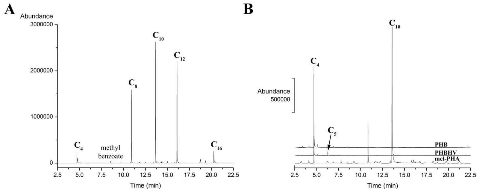
FIG. 1. Total ion chromatograms of GC-MS. (A) 3-Hydroxyalkanoic acid methyl esters derived from PHA monomer analytical standards and methyl benzoate internal standard. (B) 3-Hydroxyalkanoic acid methyl esters derived from PHA polymers PHB, PHBHV and mcl-PHA. (C 4 , C 5 , C 8 , C 10 , C 12 , C 16 represent methyl esters of 3-hydroxybutyric acid, 3-hydroxyvaleric acid, 3-hydroxyoctanoic acid, 3-hydroxydecanoic acid, 3-hydroxydodecanoic acid, and 3-hydroxyhexadecanoic acid, respectively.)
